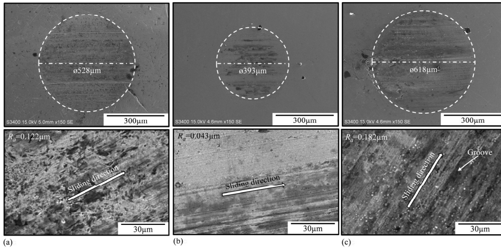
Fig. 2. SEM micrograph of worn surfaces on the ball under lubricated conditions of (a) conventional diesel engine oil, (b) with 0.5 vol. % of hBN additive, and (c) with 0.5 vol. % of Al 2 O 3 additive.
