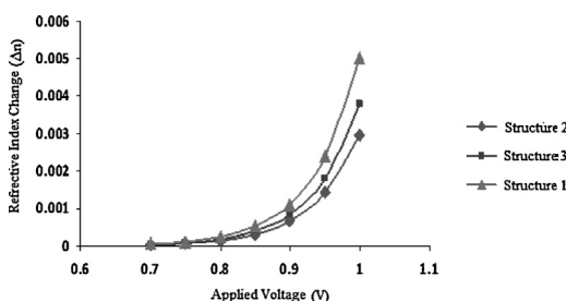
Fig. 6. Refractive index change for phase modulators with various waveguide structures.
