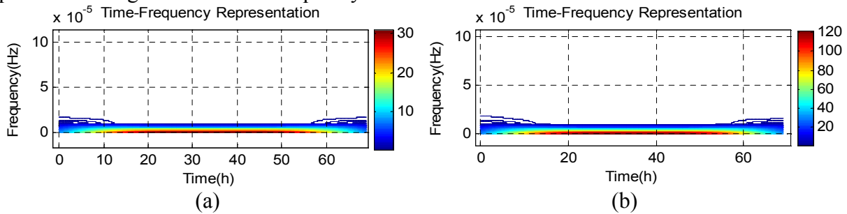
Fig. 2 Time Frequency Representation (a) 6V with 15 Ah (b) 12V with 50Ah
