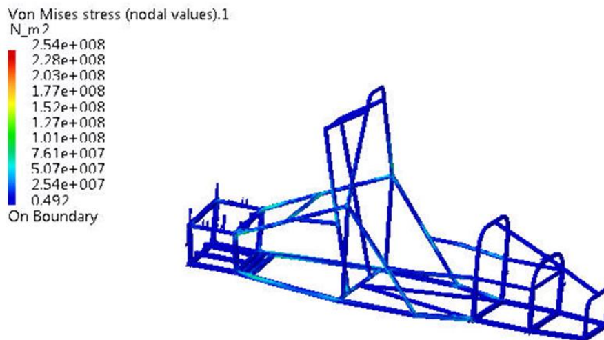
Figure 15. Stress distribution for rear stiffness analysis.
