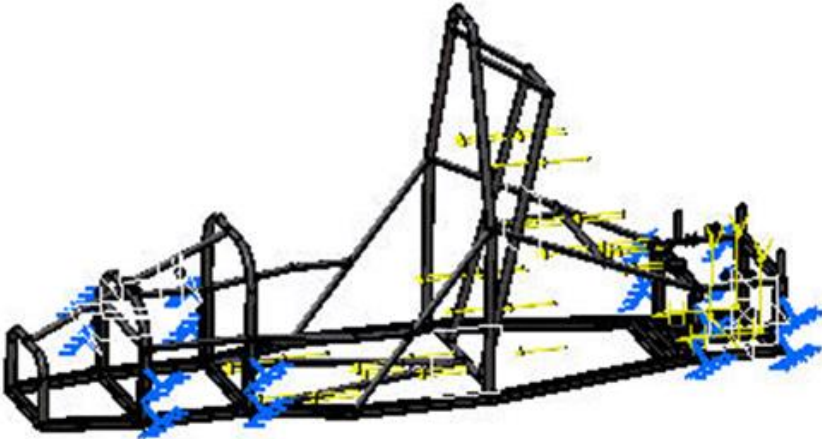
Figure 6. Braking analysis.
