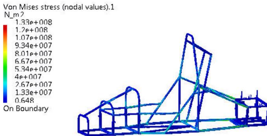
Figure 14. Stress distribution for front stiffness analysis.
