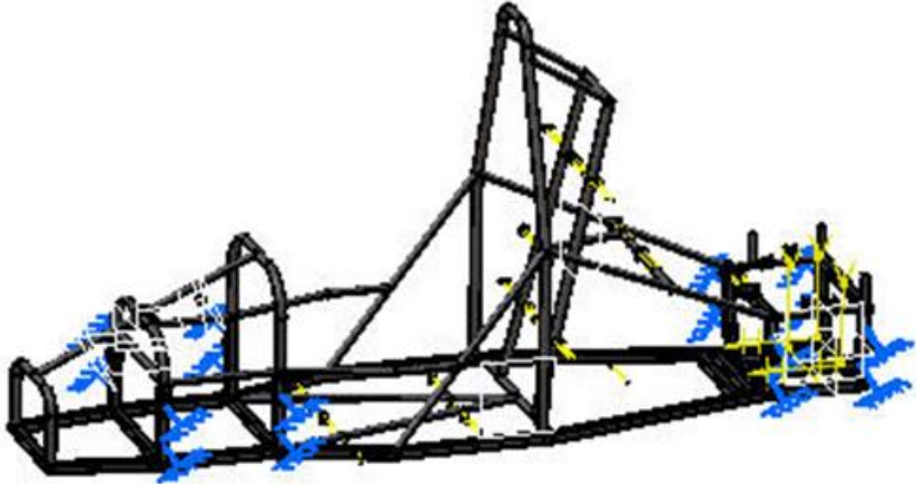
Figure 7. Cornering analysis.
