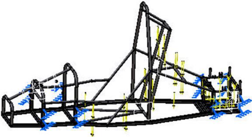
Figure 4. Static analysis.
