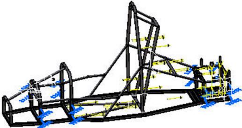
Figure 5. Acceleration analysis.
