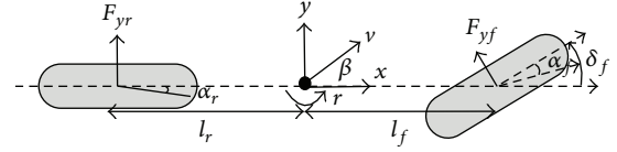
FIGURE 4: Bicycle model [31].
