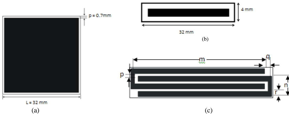
Figure 2: (a) Square (b) Rectangular (c) Halfring AMC where m = 29 mm, n = 4 mm, p = 0.5 mm, q = 1.5 mm, r = 1 mm,
