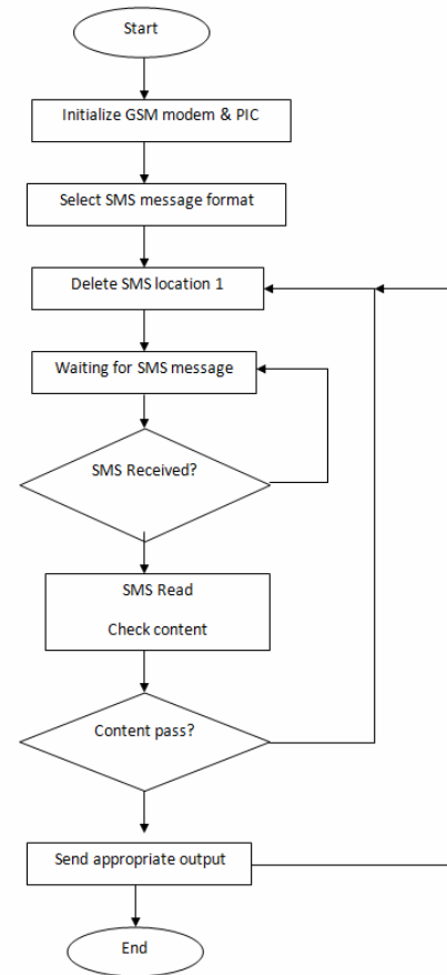
Figure-9. Flow chart of GSM.
