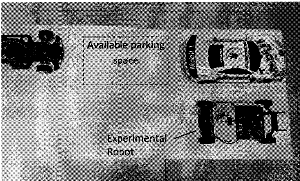
Figure 7. Parking size for adjacent distance 2.5cm
