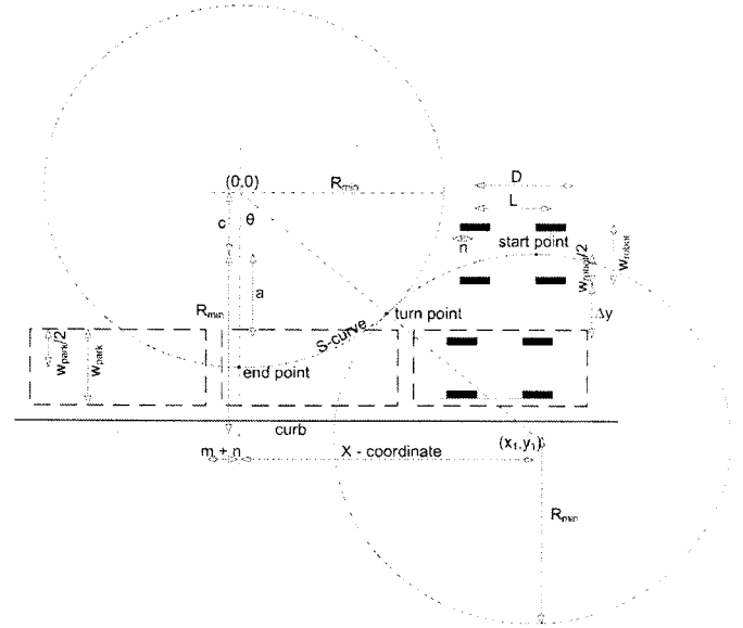
Figure 3. Path planning
