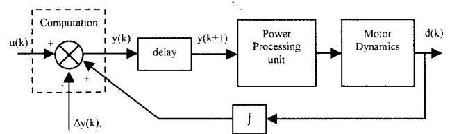
Figure 6. Control block diagram for traction system
