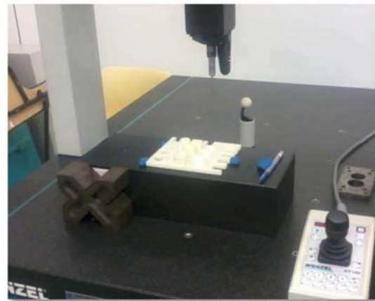
Figure-3. Measurement of part features by using the CMM.
