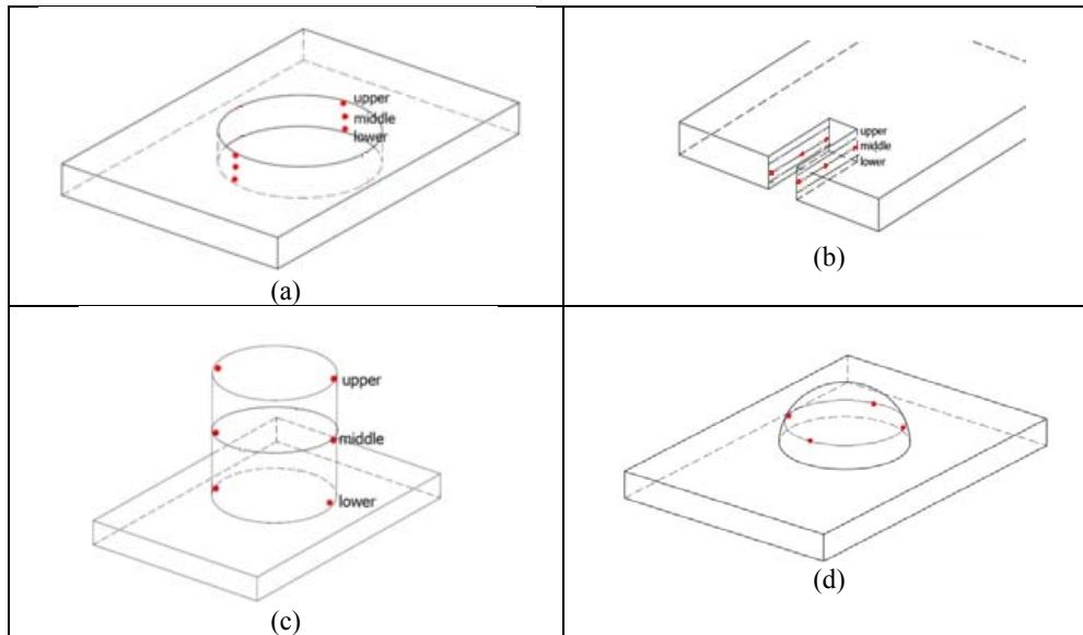
Figure-4. (a) Points of measurement for hole (b) and slot (c) cylinder (d) and sphere.
