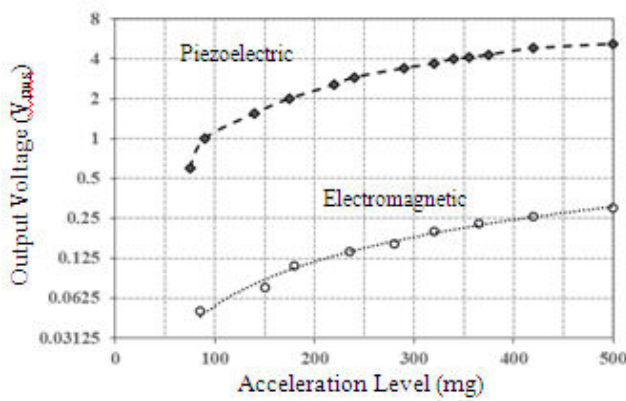
Figure- 6. Output voltage of piezoelectric and electromagnetic MGs at a range of acceleration up to 0.5g.
