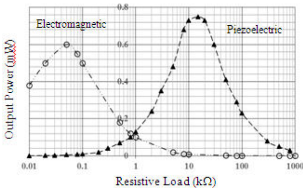
Figure-7. Output power of piezoelectric and electromagnetic MGs at resonant with an acceleration of 0.03g.
