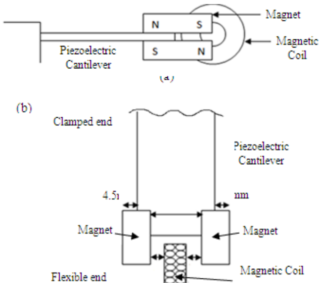
Figure-3. Schematic diagrams of (a) a side-viewed, and (b) a top-viewed electromagnetic MG attached at the end of piezoelectric cantilever with fix-positioned magnetic coil.
