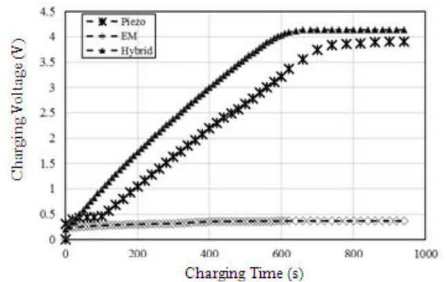
Figure-10. Capacitor charging performance of three different configurations of MGs using 16 V capacitor with capacitance of 3000 \mu F.
