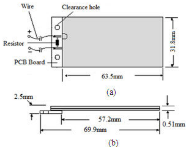
Figure-2. Q220-A4-503YB piezoelectric cantilever from Piezo System Inc, with its dimensions from (a) top view and (b) side view.
