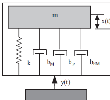
Figure-1. Second-order spring mass damper system with additional electrical damper [4].
