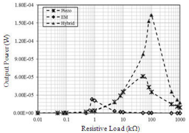
Figure-9. Rectified output power from three different configurations of MGs at varying resistive load.
