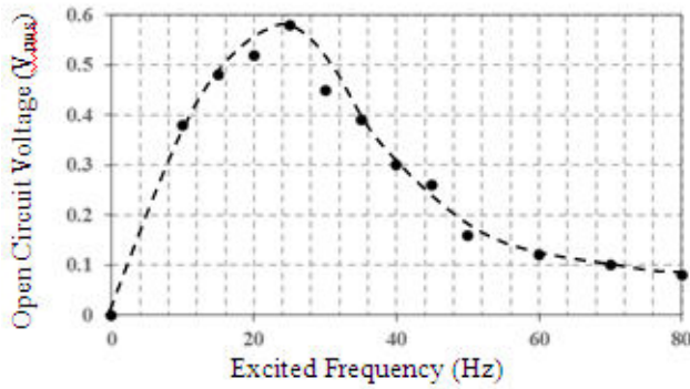
Figure-5. Frequency response of piezoelectric open circuit voltage output at an acceleration level of 0.05g.
