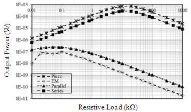
Figure-8. Output power as a function of resistive load for different configurations of MGs.
