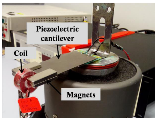
Figure-4. Photograph of hybrid MG mounted on an electrodynamic shaker.
