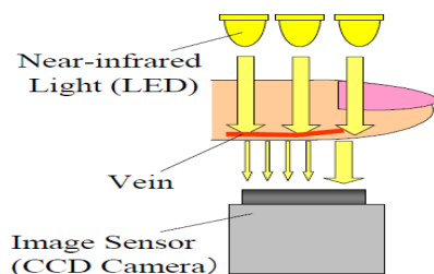
Figure-2. Light transmission method [7].
