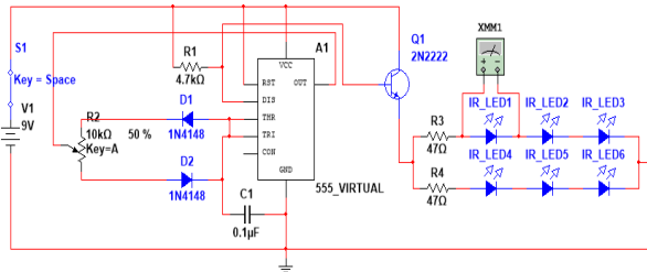
Figure-3. NIR illuminating circuit design and simulation.
