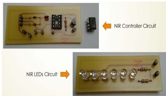
Figure-5. NIR illuminating circuit after etching and soldering.
