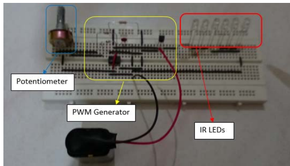
Figure-4. NIR illuminating circuit construction and testing on breadboard.
