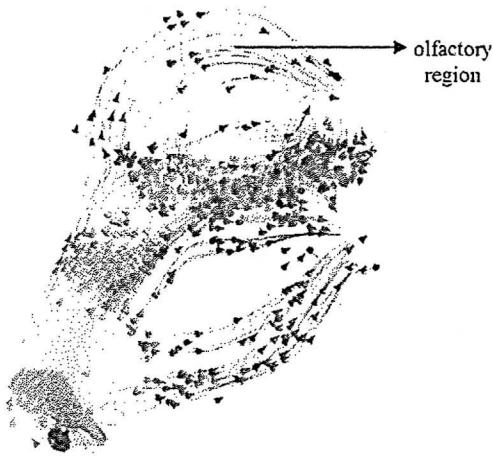
Figure.8 Fluid particle trajectories for healthy model.
