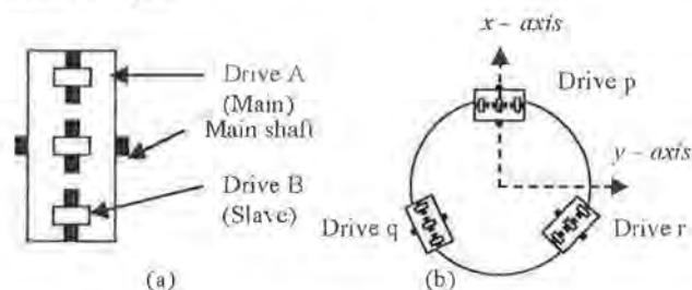
Figure 1. Wheel configuration
