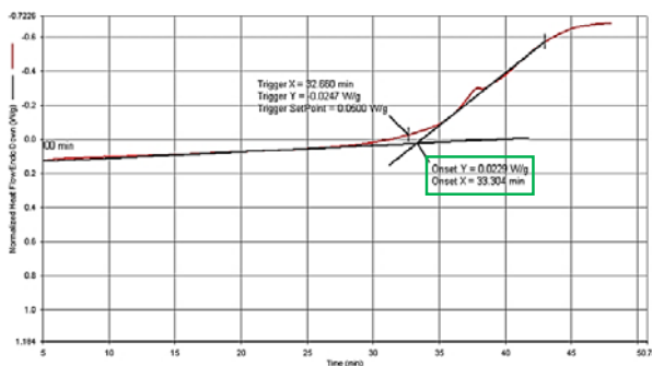
Figure-6. OIT response of optimized NEI oil (OIT is 33 minutes).
