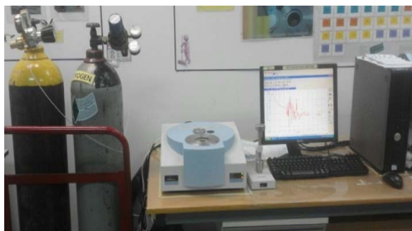
Figure-1. Perkin Elmer Jade DSC equipment for OIT test.
