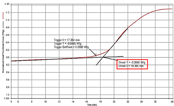
Figure-5. OIT response of fresh NEI oil (OIT is 18 minutes).
