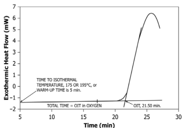
Figure-2. Example of hydrocarbon oil oxidation under OIT test (OIT is determined as a time which intersection occur between base line and tangential line of the rising exotherm) [29].
