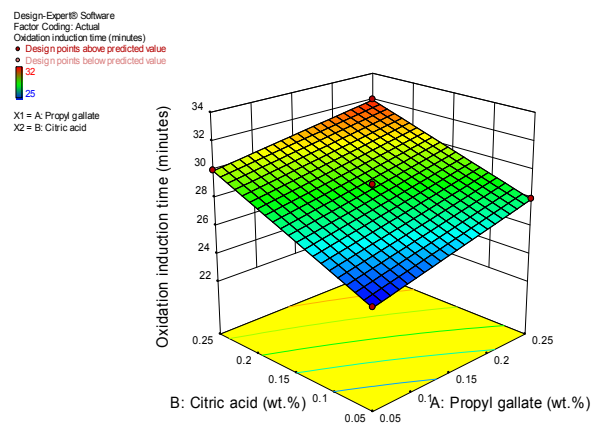
Figure-4. Response surface plot which shows the effect of the propyl gallate and citric acid concentrations on the oxidation induction time.
