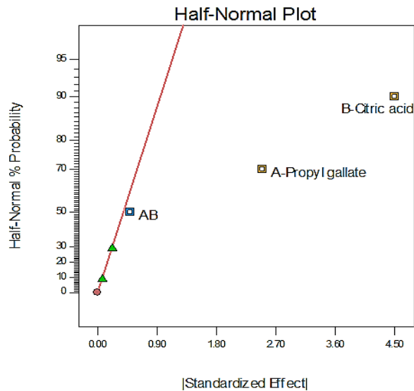
Figure-3. Half-normal plot obtained from the 2^2 factorial design of experiments.
