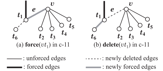
Fig. 21 Illustration for c-11 where vertices v \in V_{u5} and t_1 \in N_U(v; V_{f3}) .
