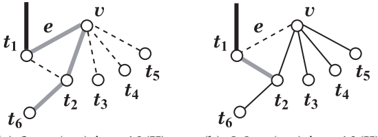
Fig. 16 Illustration for c-10(II) where vertices v \in V_{u5} and t_1 \in N_U(v; V_{f3}) , such that N_U(v) \cap N_U(t_1) = \{t_2\} , t_2 is a u3-vertex, and the unique neighbor of t_2 not in \{t_1, v\} is in N_U(v) .
