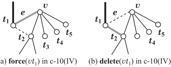
Fig. 19 Illustration for c-10(IV) where vertices v \in V_{u5} and t_1 \in N_U(v; V_{f3}) , such that N_U(v) \cap N_U(t_1) = \{t_2\} , t_2 is a u4-vertex.
