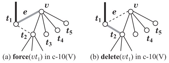
Fig. 20 Illustration for c-10(V) where vertices v \in V_{u5} and t_1 \in N_U(v; V_{f3}) , such that N_U(v) \cap N_U(t_1) = \{t_2\} , t_2 is a u5-vertex.
