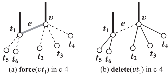
Fig. 6 Illustration of branching rule c-4, where vertex v \in V_{f5} and vertex t_1 \in N_U(v; V_{f4}) , such that N_U(v) \cap N_U(t_1) = \emptyset .
