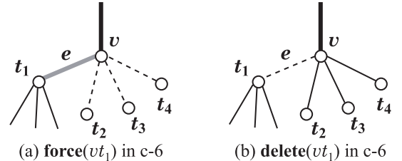
Fig. 9 Illustration of branching rule c-6, where vertex v \in V_{f5} and vertex t_1 \in N_U(v; V_{u4}) .
