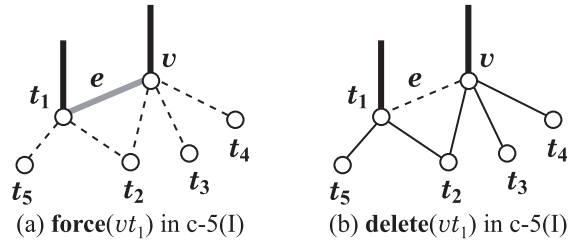
Fig. 7 Illustration of branching rule c-5(I), where vertex v \in V_{f5} and vertex t_1 \in N_U(v; V_{f4}) , such that N_U(v) \cap N_U(t_1) = \{t_2\} .
