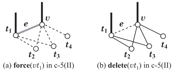
Fig. 8 Illustration of branching rule c-5(II), where vertex v \in V_{f5} and vertex t_1 \in N_U(v; V_{f4}) such that N_U(v) \cap N_U(t_1) = \{t_2, t_3\} .
