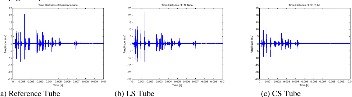
Fig. 5: Typical stress wave history of the inspected tubes.
