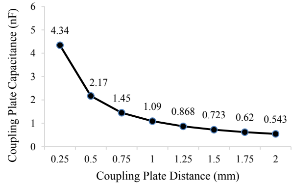
Fig.10. Capacitance vs. Distance.
