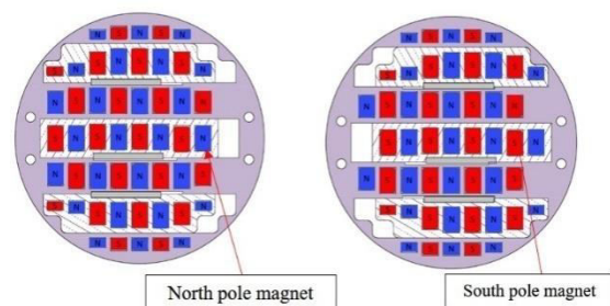
Figure-22. Arrangement of the magnet.
