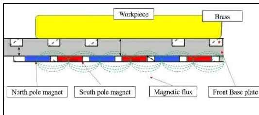
Figure-23. The thickness the magnetic clamping.
