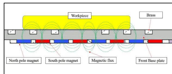
Figure-21. Magnet flux flow in the magnetic clamping.
