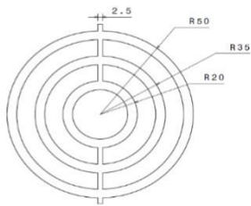
Figure-10. Dimension of the brass.
