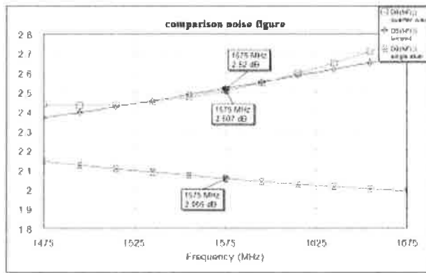
Fig. 10: Comparison of Noise Figure.
