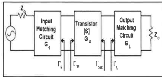
Fig. 3: The General Transistor Amplifier Circuit.
