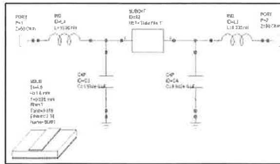
Fig. 7: Lumped Element Matching Network.
