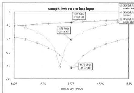
Fig. 8: Comparison Return Loss Input (S11).
