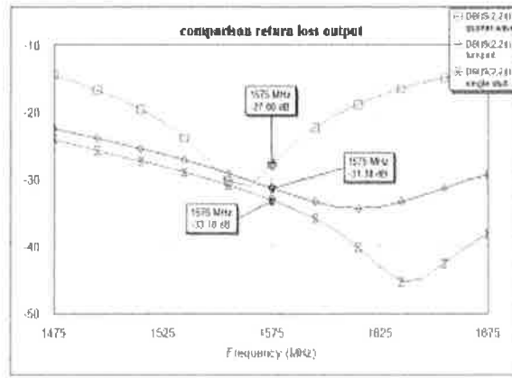
Fig. 9: Comparison Return Loss Output (S22).
