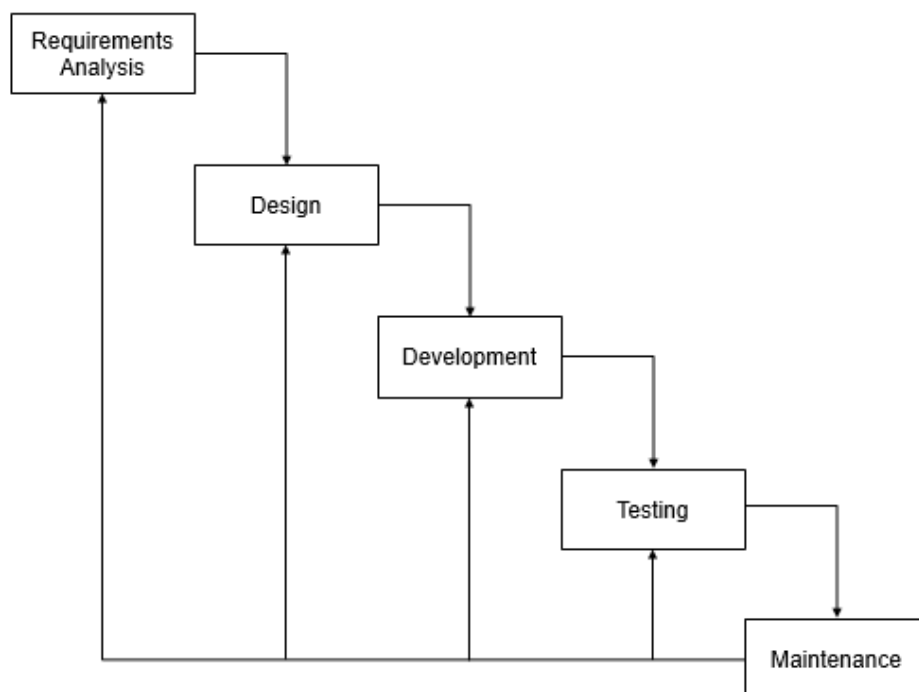
Figure 1.1: Waterfall Model
