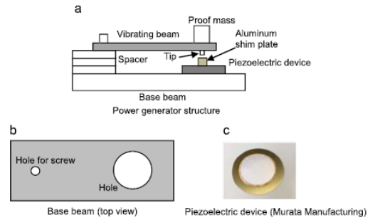
Figure 11: The power generator, base beam and piezoelectric device [30].
