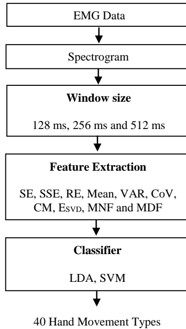
Fig. 1 - Flow diagram of the pattern recognition architecture.
