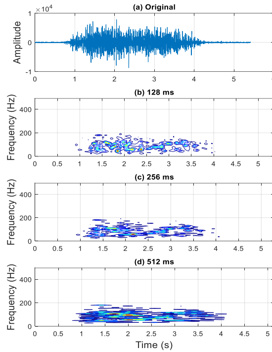
Fig. 2 - Spectrogram of EMG signal with three different Hanning window sizes. (a) EMG signal (b) 128 ms (c) 256 ms (d) 512 ms.
