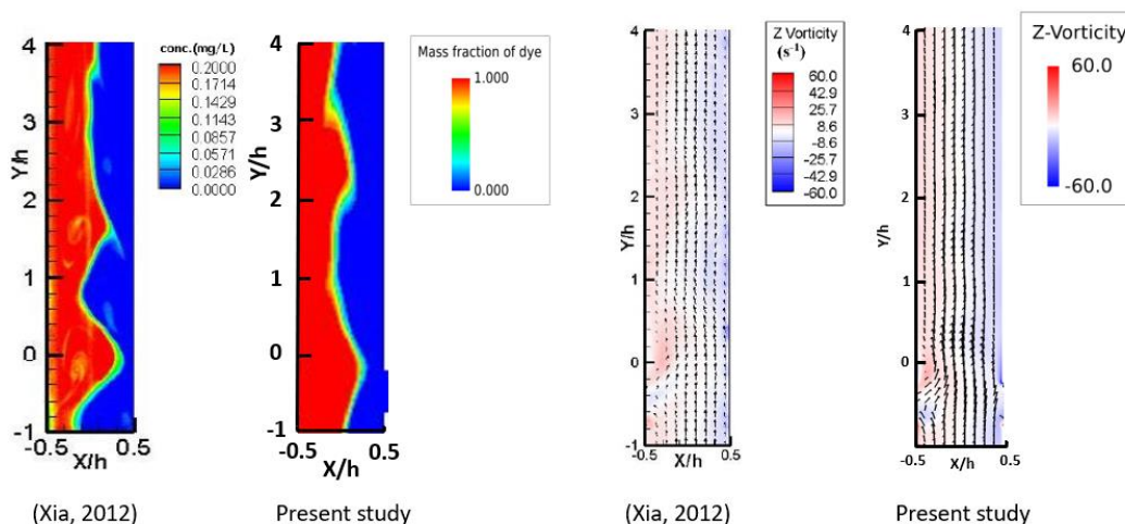
Fig. 11. Comparison between instantaneous concentration contours (left), and phase-averaged velocity vector and vorticity contours (right) obtained from experiment and present study. All the visualization results are captured near the orifice exit region at the end of ejection cycle of left SJA under stroke ratio, L = 2 and velocity ratio, R_v = 0.8
