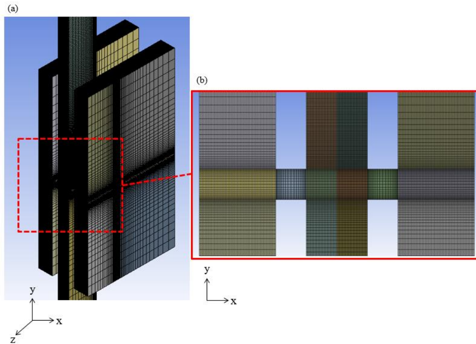
Fig. 3. Meshed model for present study (a) View of three-dimensional (b) View of two-dimensional
