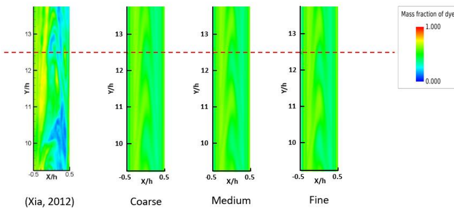
Fig. 6. Comparison of instantaneous concentration contours around the region of evaluation plane (red dot line) among experiment and three different meshes at stroke ratio, L = 4 and velocity ratio, R_v = 1.6
