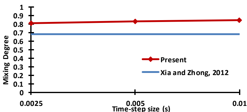
Fig. 7. Comparison of time-averaged mixing degree obtained from different time-step sizes ( t=0.0025, 0.005, 0.01 s) and experiment at stroke ratio, L = 4 and velocity ratio, R_v = 1.6
