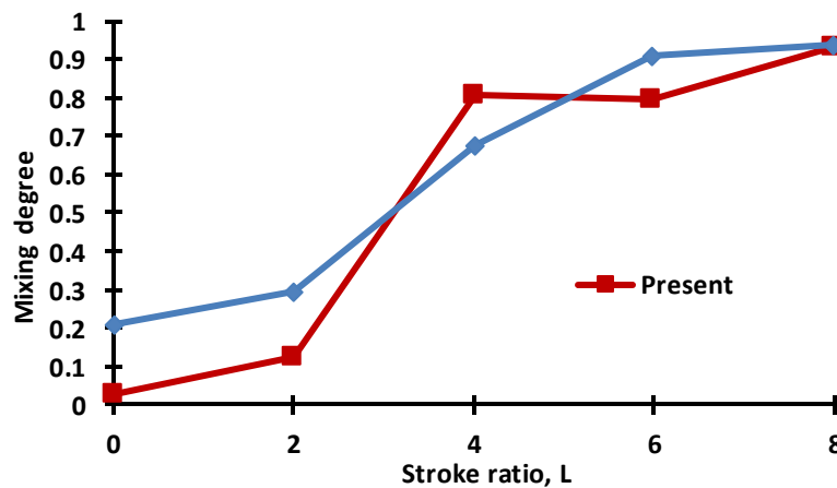
Fig. 10. Comparison of time-averaged mixing degree obtained from experiment and present study at different Stroke ratio, L
