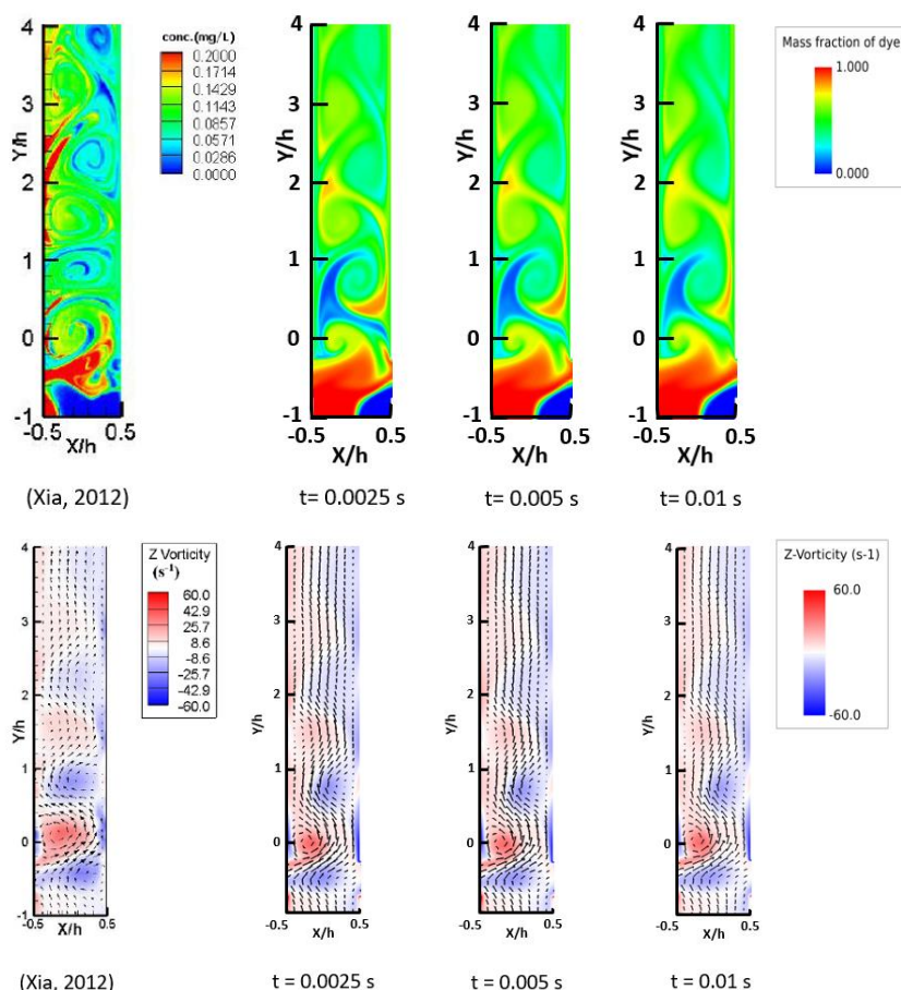
Fig. 8. A comparison of instantaneous concentration contours (upper), and phase-averaged velocity fields and vorticity contours (bottom) among experiment and different time-step sizes. All the visualization results are captured around the orifice exit region at the end of ejection cycle of left SJA under stroke ratio, L = 4 and velocity ratio, R_v = 1.6
