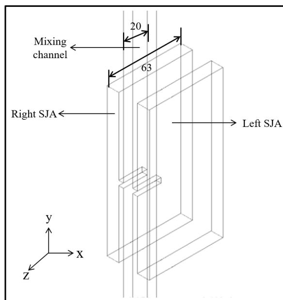
Fig. 2. A 3D schematic diagram of the geometric model
