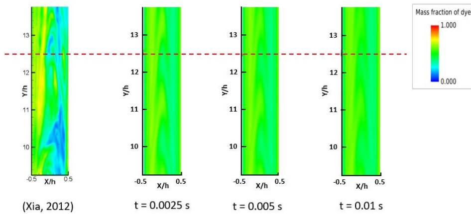
Fig. 9. A comparison of instantaneous concentration contours around the region of evaluation plane (red dot line) among experiment and different time-steps at stroke ratio, L = 4 and velocity ratio, R_v = 1.6
