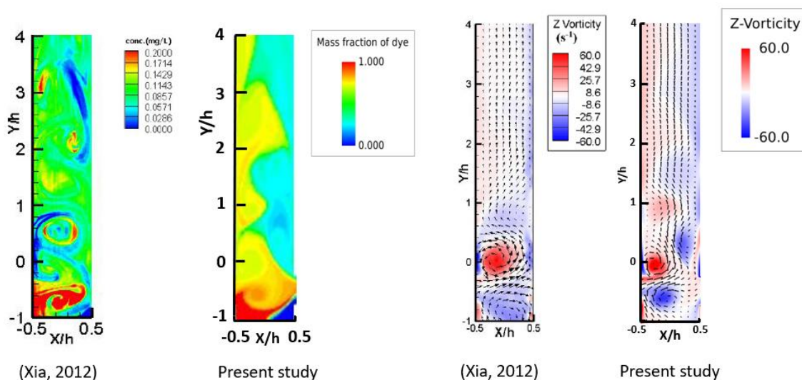
Fig. 12. Comparison between instantaneous concentration contours (left), and phase-averaged velocity vector and vorticity contours (right) obtained from experiment and present study. All the visualization results are captured near the orifice exit region at the end of ejection cycle of left SJA under stroke ratio, L = 6 and velocity ratio, R_v = 2.4
