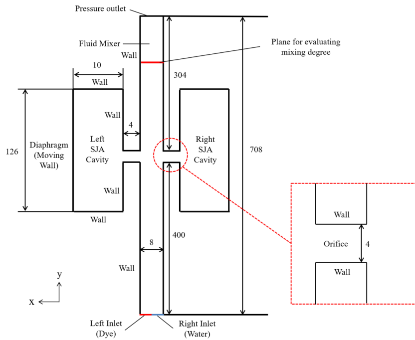
Fig. 1. 2D Schematic diagram of the geometric model
