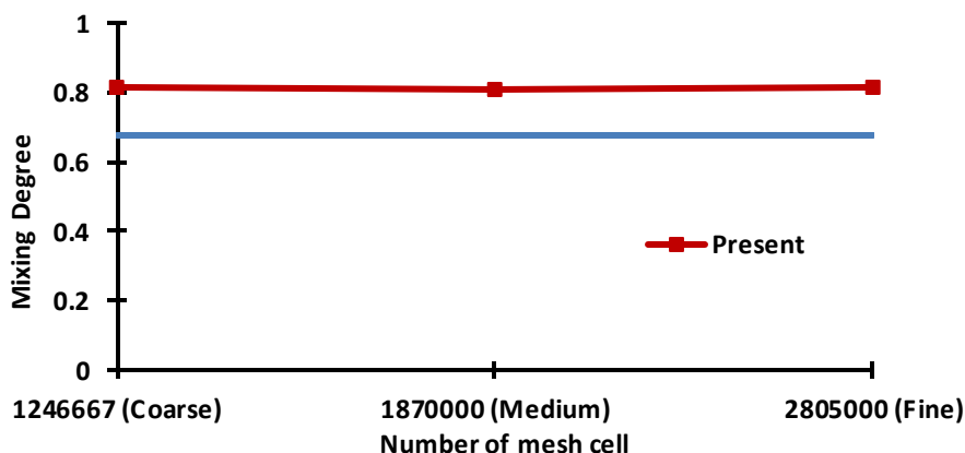
Fig. 4. Comparison of time-averaged mixing degree obtained from different mesh refinement cases and experiment at stroke ratio, L = 4 and velocity ratio, R_v = 1.6
