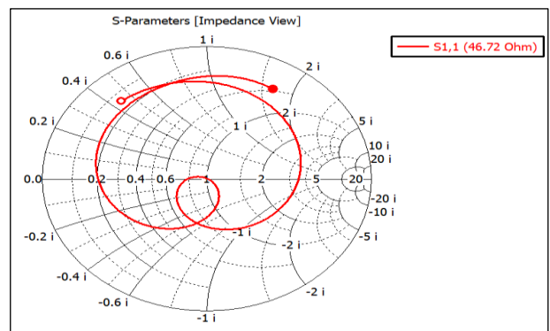
Figure 13: The impedance matching of 4x1 array antenna
