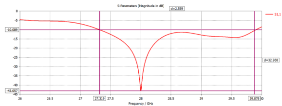
Figure 5: The return loss of 8x1 array antenna
