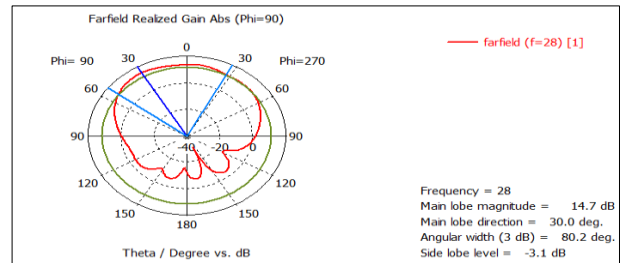
Figure 11: Radiation pattern of 8x1 array antenna
