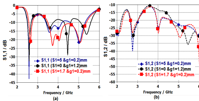
Figure 11: S-parameters of the crescent slot MIMO antenna with changing values of the gap g_1 and S_1 , while fixing L_g = 8.2 mm and L_f = 12.78 mm (a) Simulated return loss (b) Simulated isolation.
