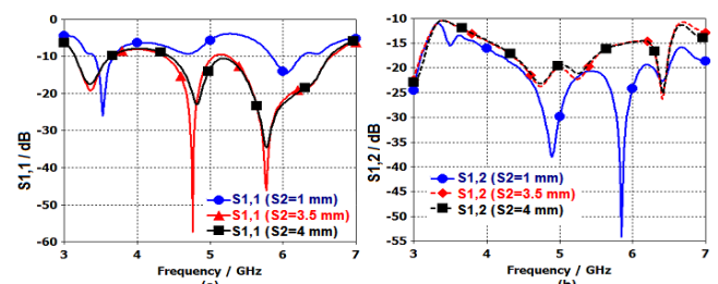
Fig. 5: S-parameters of the crescent slot MIMO antenna with changing values of S2 while fixing L_g = 8.2 mm, L_f = 12.78 mm. (a) Simulated return loss (b) Simulated isolation
