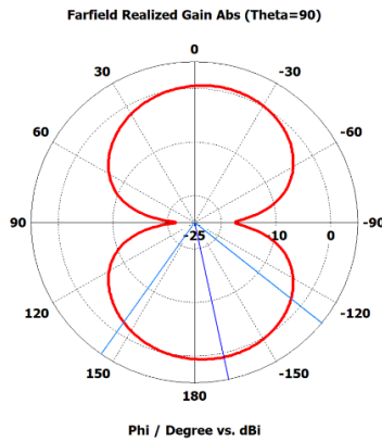
Fig 8. E-Plane radiation pattern
