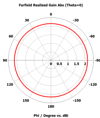
Fig 9. H-Plane radiation pattern
