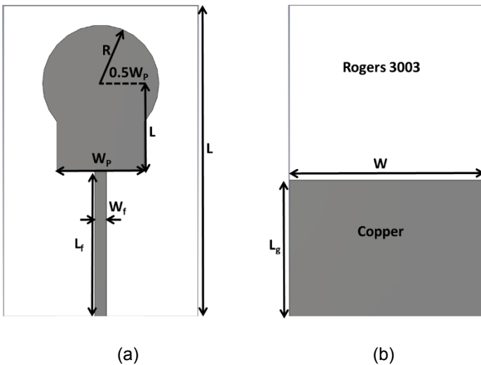
Fig 1. (a) the front and (b) the back view of the antenna ( R=6 mm, W_p=L_p=9 mm, L_f=15 mm, W_f=1.2 mm, L_g=14 mm, W=20 mm and L=32 mm)
