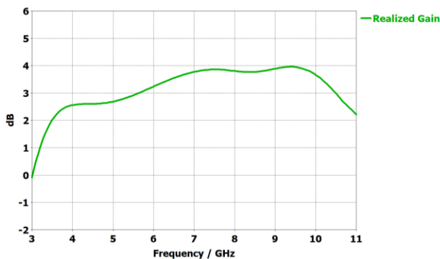
Fig 10. Realized gain Vs frequency
