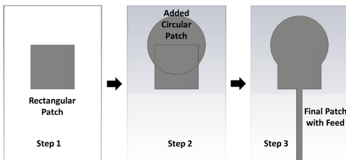
Fig 2. Steps of the antenna structure design
