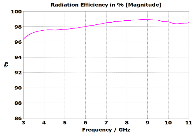
Fig 6. The radiation efficiency of the antenna
