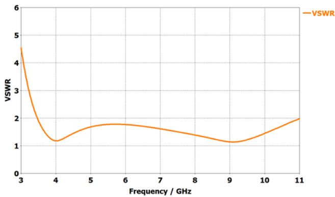
Fig 4. VSWR response of the antenna
