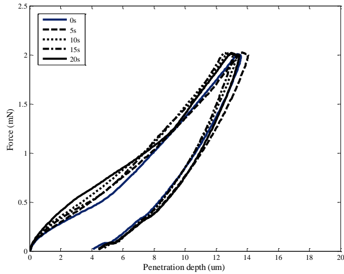
Figure 8. The graph of nano-indentation curve for 20 phr with various hold times.
