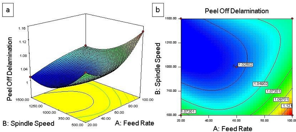
Figure 4. 3D response surface plot of peel off delamination; (a) coupled with its contour plots (b) as a function of feed rate and spindle speed.
