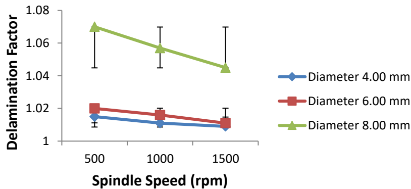
Figure 2. Effect of drill diameter with respect to the spindle speed on delamination factor.
