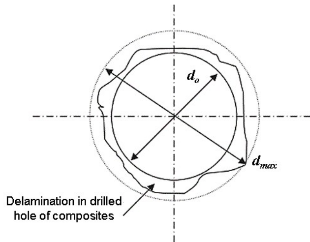
Figure 1: Schematic diagram showing the measurement of delamination diameter, d , induced by drilling of composites [21].
