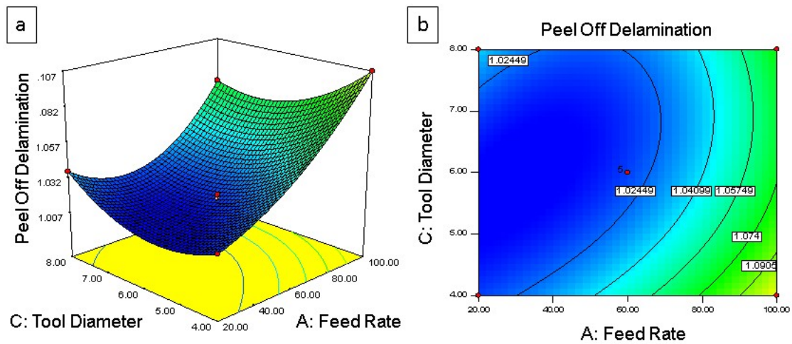
Figure 5. 3D response surface plot of peel off delamination (a) coupled with its contour plots (b) as a function of feed rate and tool diameter.
