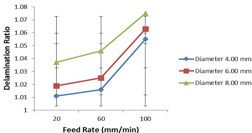
Figure 3. Effect of drill diameter with respect to the feed rate on delamination factor.
