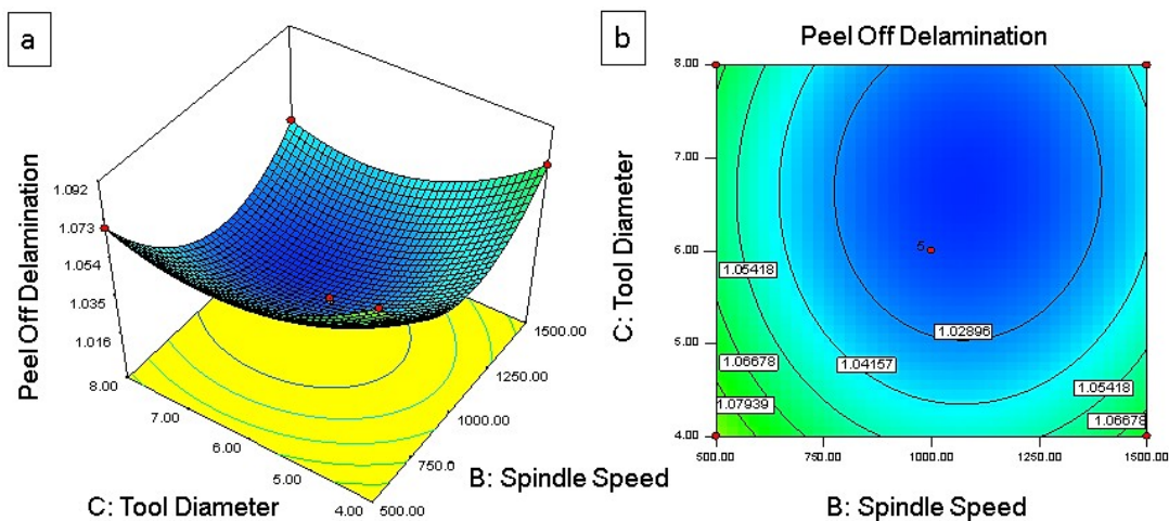
Figure 6. 3D response surface plot of peel off delamination (a) coupled with its contour plots (b) as a function of spindle speed and tool diameter.
