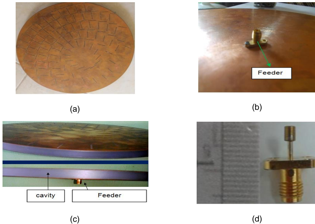
Figure 3. (a) Front View of the Prototype; (b) Back View of the Prototype; (c) Side View of the Prototype; (d) Structure of Feeder
