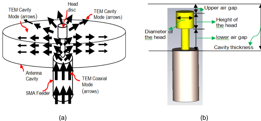
Figure 2. (a) Signal Flow of RLSA antennas (b) Feeder
