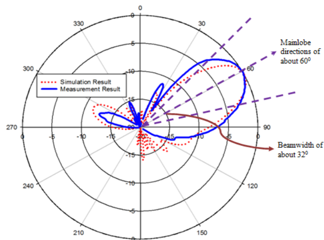
Figure 6. Simulated and Measured Radiation Pattern
