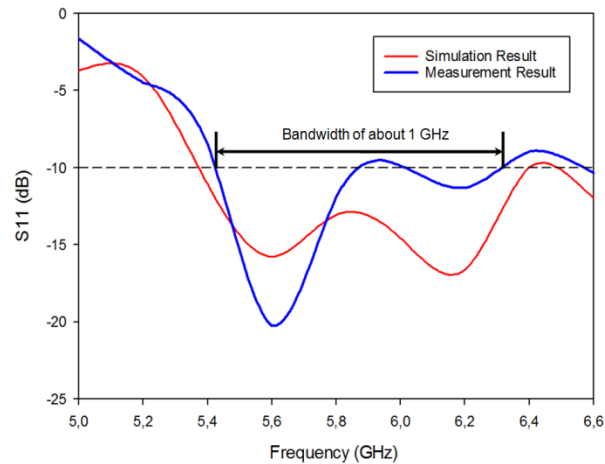
Figure 5. Simulated and Measured S_{11}
