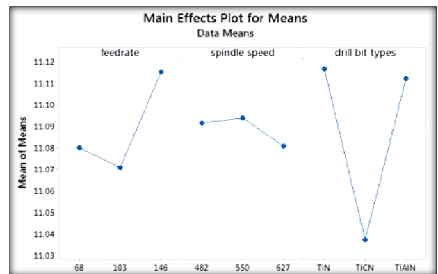
Figure 2: Main Effect Plots for Means
