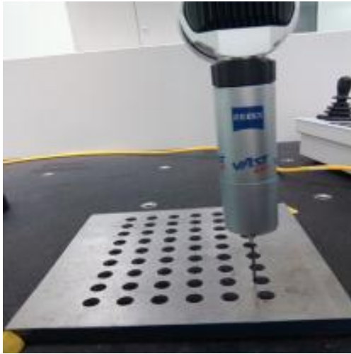
Figure 2: Hole diameter measurement
