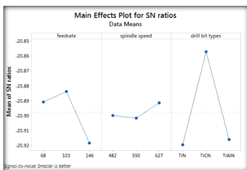
Figure 1: Main Effect Plots for SN Ratios
