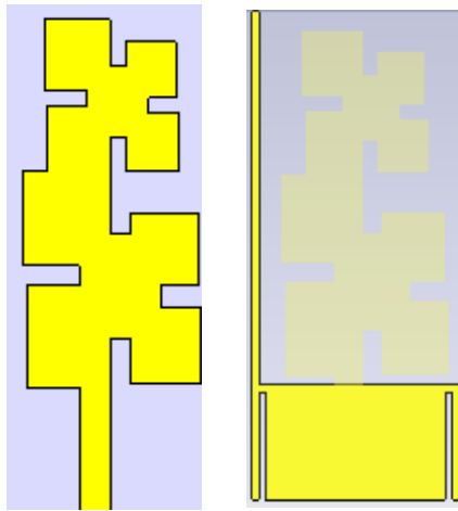
Fig.1: A Fractal Sierpinski single antenna
