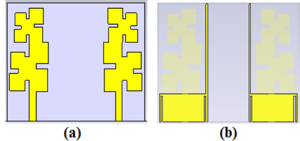
Fig.4: Fractal MIMO antenna (a) Patch plane (b) Ground plane
