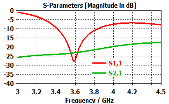
Fig. 5: S-Parameters of the Sierpinski MIMO antenna
