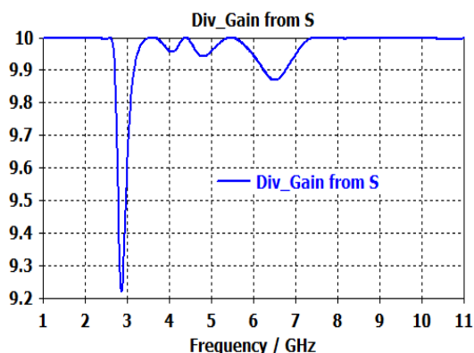
Fig. 8: DG of Disc MIMO Antenna
