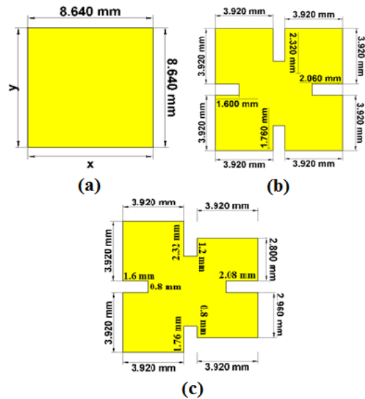
Fig.3: configuration of fractal antenna (a) iniatior antenna , (b) 0 th iteration (c) modified patch
