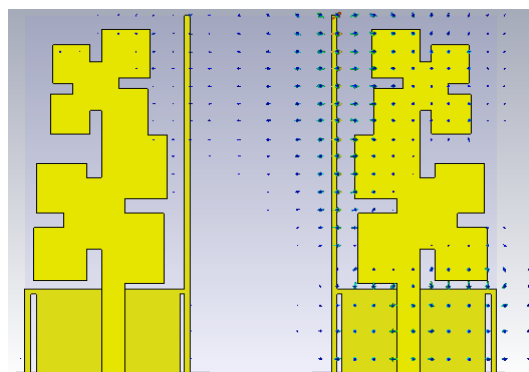
Fig. 9: Simulated current densities with port1 of the fractal Sierpinski MIMO antenna (a) Top view (b) Back view
