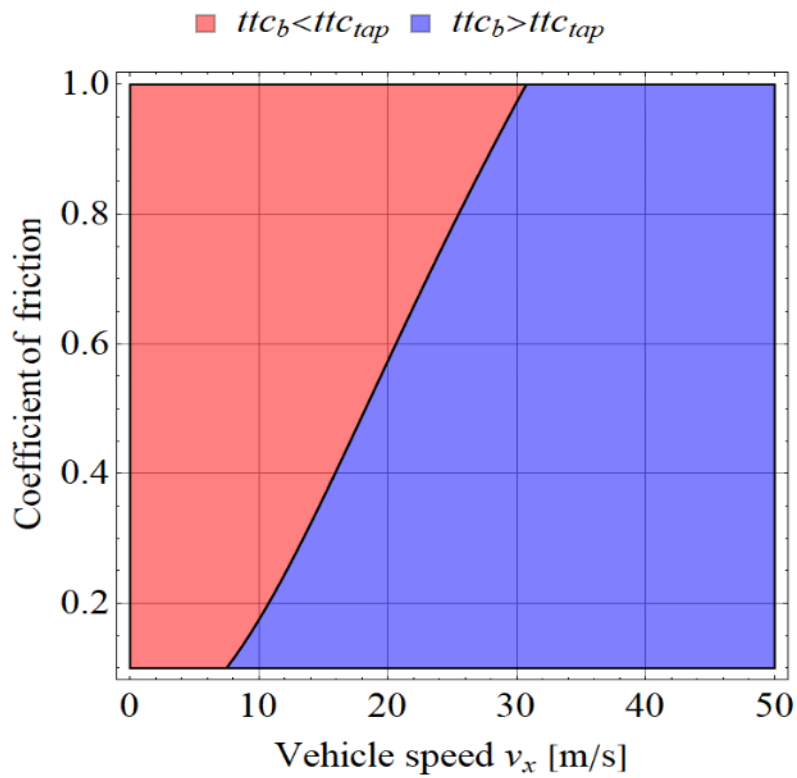
Figure 11: Regions in which either braking or steering avoidance gives the shortest time to collision at which the avoidance maneuver must be initiated to avoid collision for trapezoidal acceleration profile
