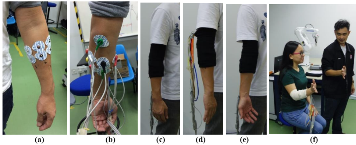
Fig 4 - The positions of the electrodes (a) front view (b) rear view, arm position (c) neutral (d) supination (e) pronation (f) general view of procedure during recording.
