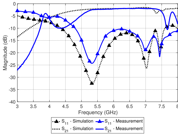
FIGURE 7. Scattering parameters of the probe-to-probe setup.
