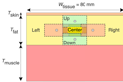
(a) Cross-view shows different misalignment scenarios between the probes.
