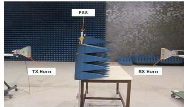
Fig.7. The photo of the measurement setup.
