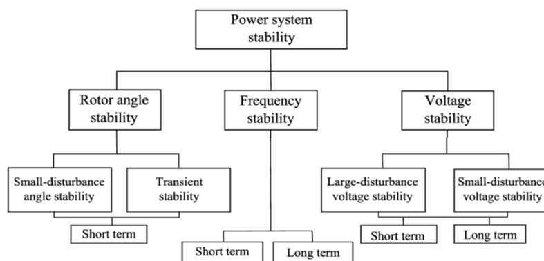
Figure 1. Classification of power system stability
