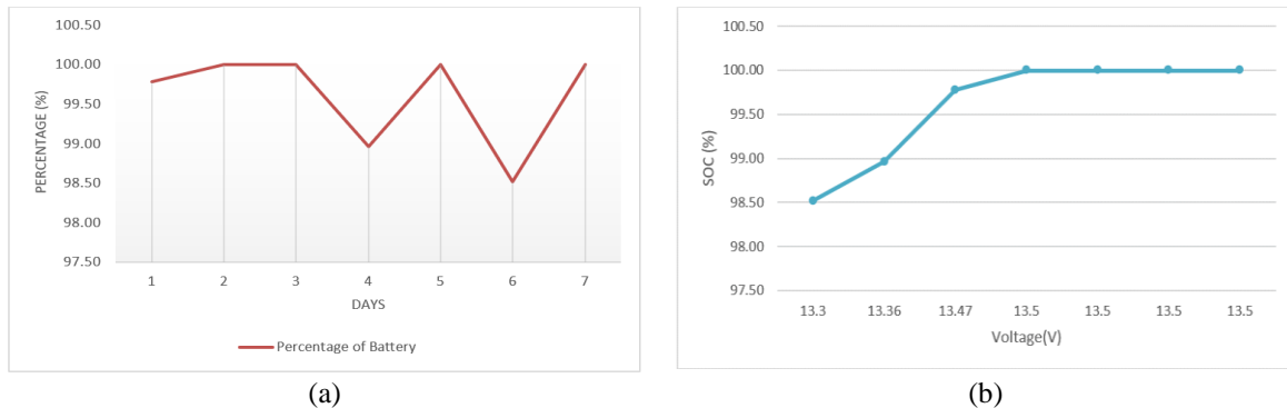
Figure 11. There figures are; (a) SOC vs days; (b) SOC vs voltage
