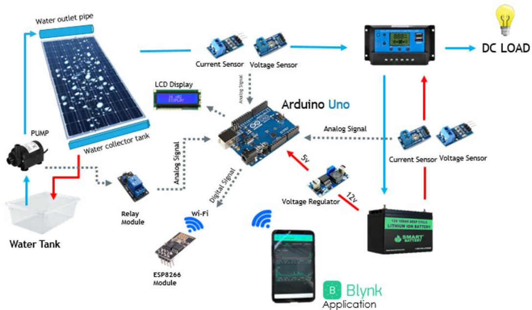
Figure 5. System configuration
