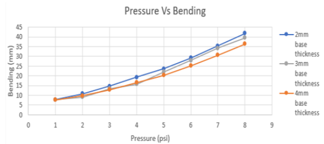
(b) Pressure vs. bending elongation
