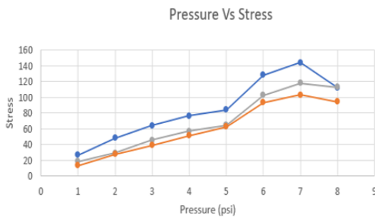
(a) Pressure vs. von mises stress
