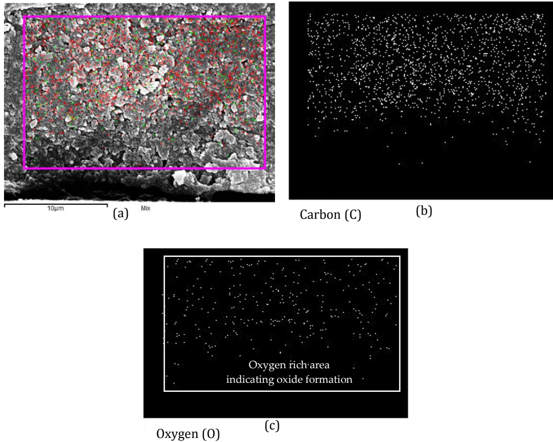
Figure 9: EDX Mapping Images with Oxygen Rich Area Indicating Oxide Formation of 20 Minutes Curing Time. (a) SEM Image, (b) EDX Mapping Image of Carbon (graphene), (c) EDX Mapping Image of Oxygen.
