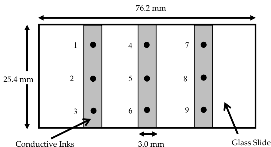
Figure 1. Schematic of printed CI on a glass slide with 9 marking points for electrical measurement.
