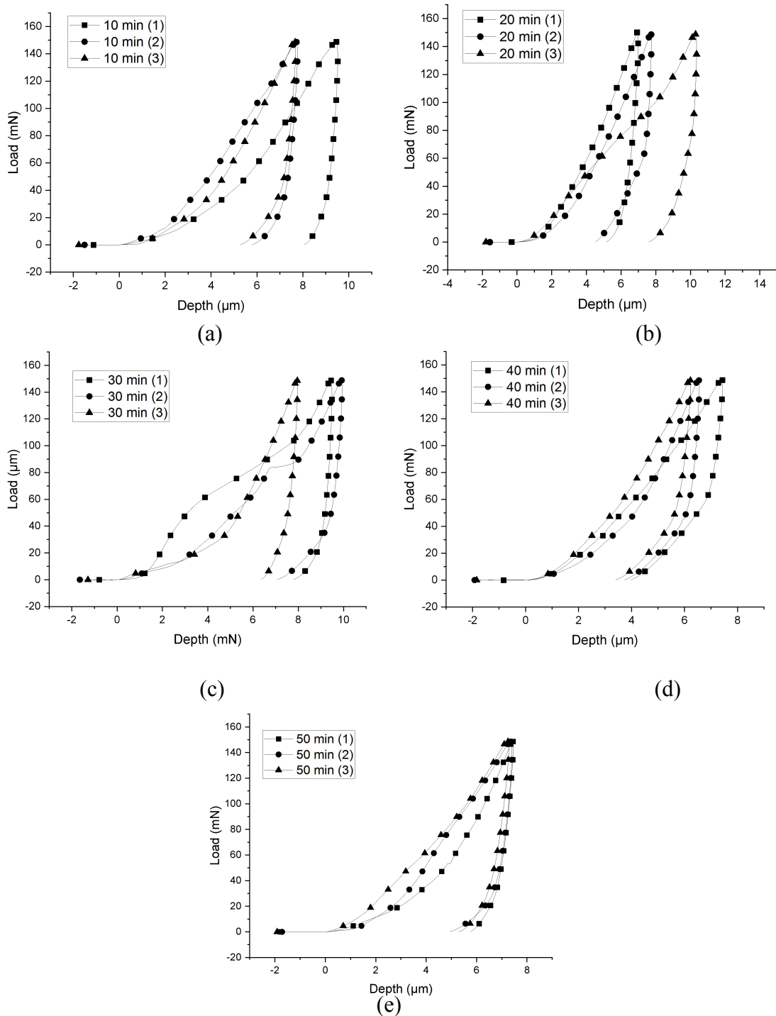
Figure 4. Representation of load–displacement curves showing different penetration depths, (a) 10 minutes, (b) 20 minutes (c) 30 minutes, (d) 40 minutes, (e) 50 minutes.
