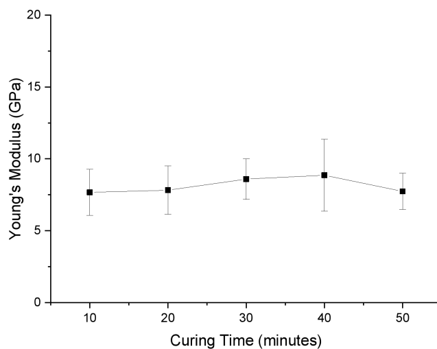
Figure 5. Mean values of filler loading curing time Young's modulus.
