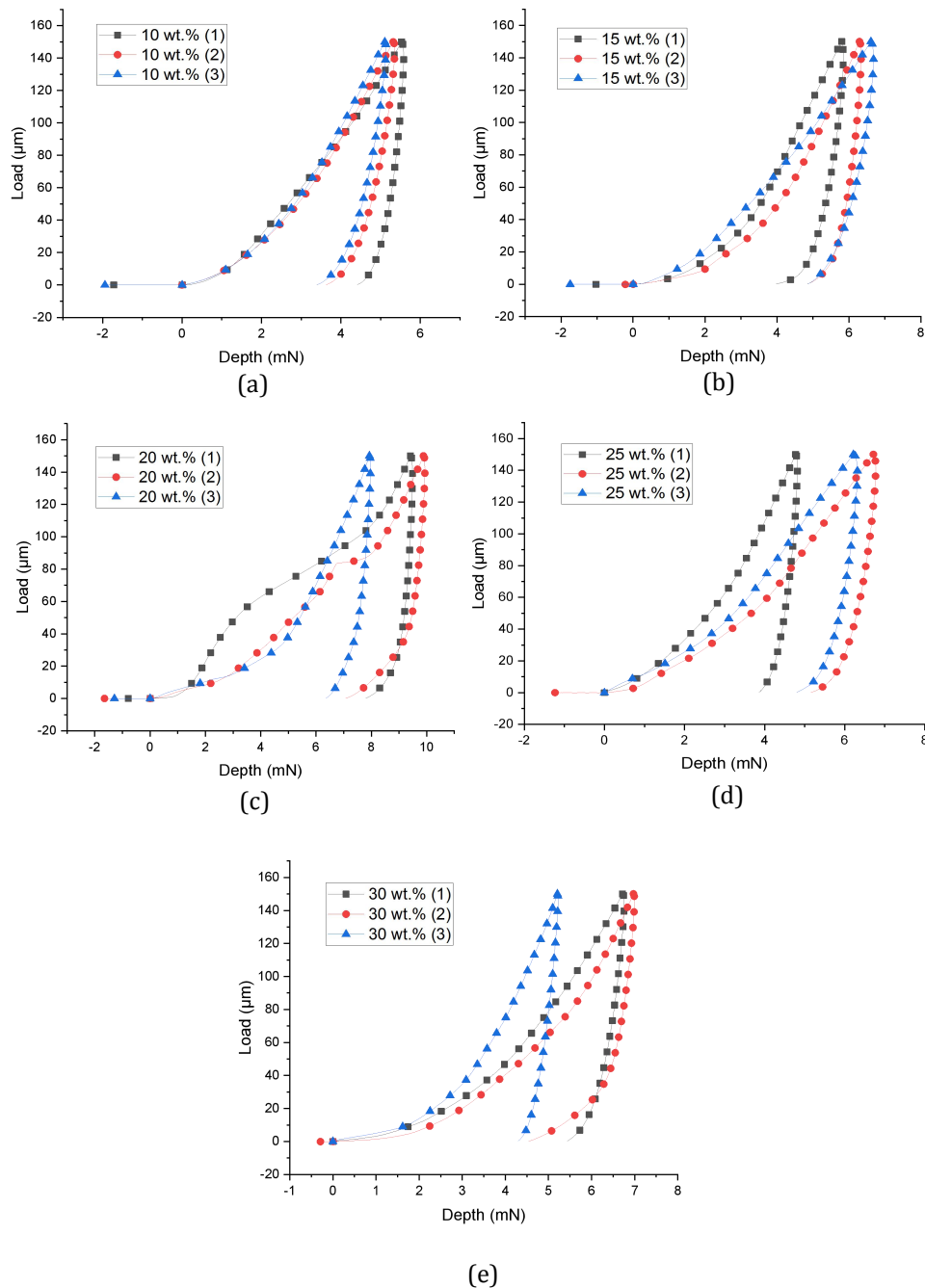
Figure 5. Representation of load–displacement curves showing different penetration depths, (a) 10 wt%, (b) 15 wt.%, (c) 20 wt.%, (d) 25 wt.% and (e) 30 wt.%.
