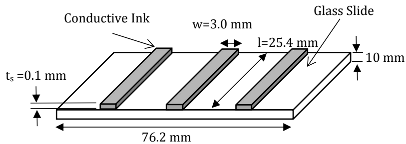
Figure 3. Pattern of thick layer dimension of conductive ink on the glass slide.
