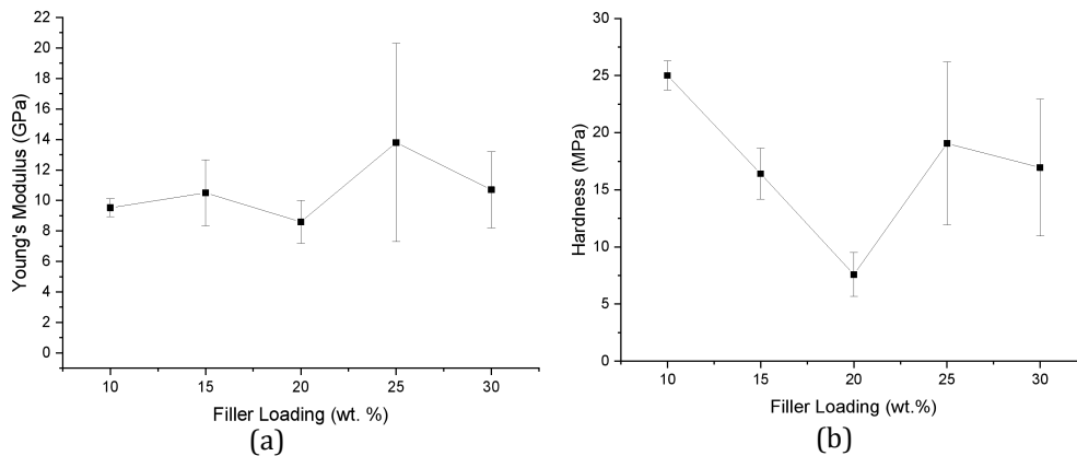
Figure 6. Mean values of (a) Young's modulus of elasticity and (b) hardness versus filler loading percentages.
