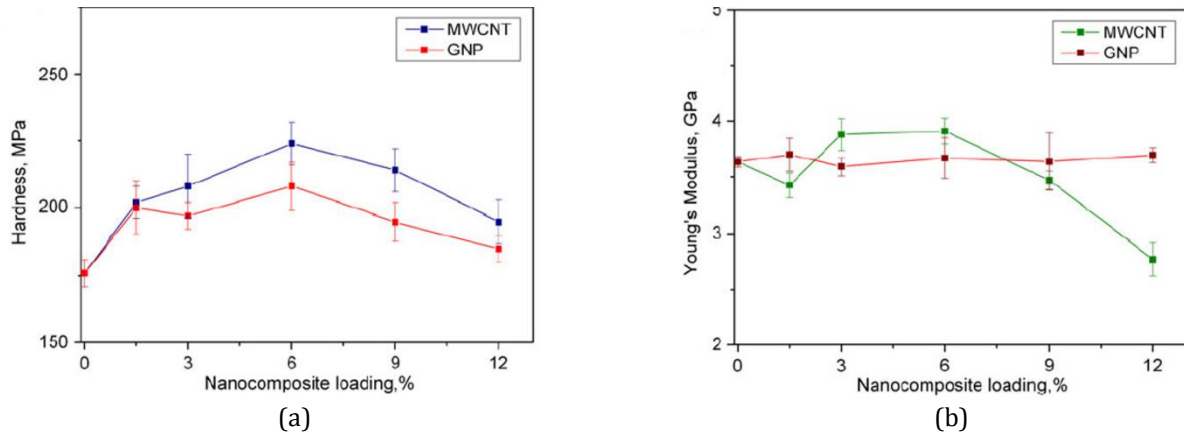
Figure 2. Mean values of (a) hardness and (b) Young's modulus of elasticity versus mono-filler content [8].
