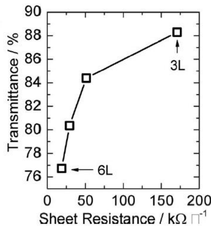
Figure 1. Graphene sheet resistance [7].
