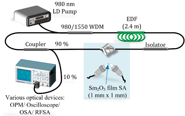
Fig. 3. Schematic configuration of Q-switched EDFL (color online)
