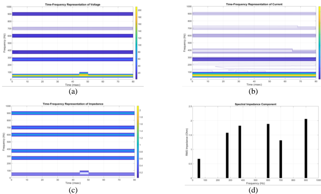
Figure 7. Case 3: (a) voltage signal in TFR using S-transform, (b) current signal in TFR using S-transform, (c) TFR impedance using S-transform, and (d) spectral impedance
