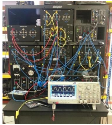
Figure 4. Experimental setup of the proposed system
