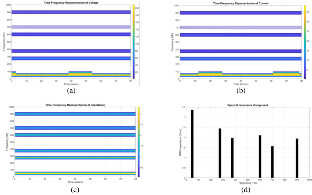
Figure 6. Case 2: (a) voltage signal in TFR using S-transform, (b) current signal in TFR using S-transform, (c) TFR impedance using S-transform, and (d) spectral impedance
