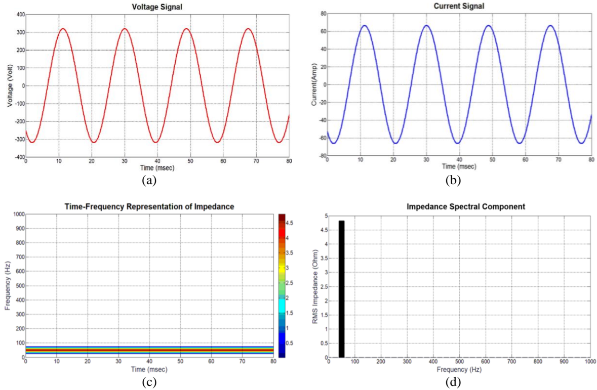
Figure 5. Case 1: (a) voltage signal in time domain, (b) current signal in time-domain, (c) TFR impedance using S-transform, and (d) spectral impedance
