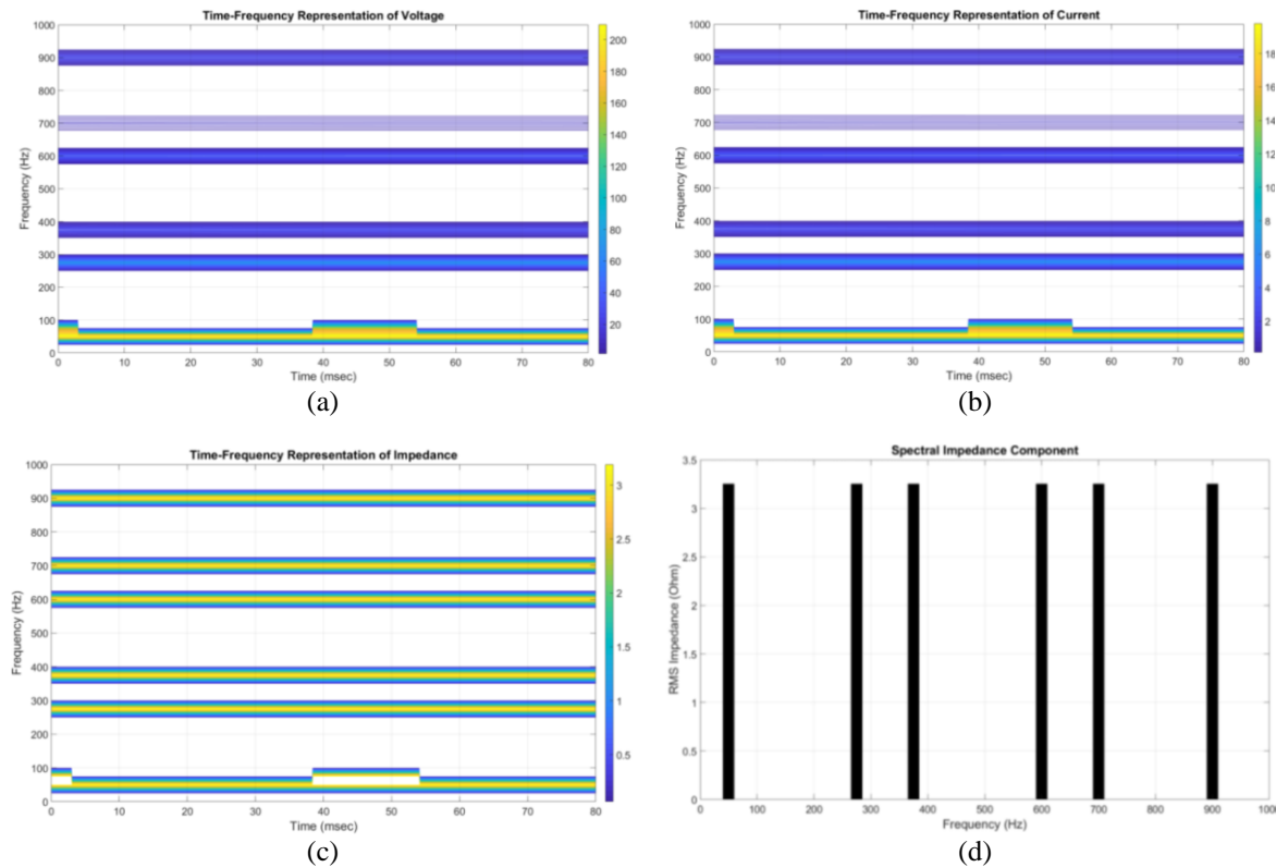
Figure 8. Case 4: (a) voltage signal in TFR using S-transform, (b) current signal in TFR using S-transform, (c) TFR impedance using S-transform, and (d) spectral impedance (Z S )
