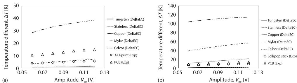
Figure 4. The impact of stack's material on temperature drops across stack length of (a) 4 cm and (b) is 8 cm long inside resonator of 0.65 m long
