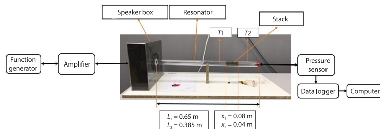
Figure 2. The experimental apparatus of the thermoacoustic cooler
