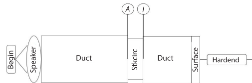
Figure 1. Schematic diagram of segments as defined in DeltaEC software
