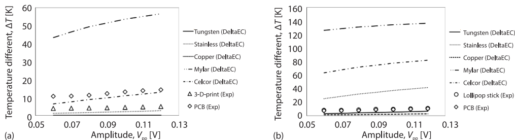
Figure 5. The impact of stack's material temperature drop across stack length of (a) 4 cm and (b) is 8 cm long inside resonator of 0.385 m long
