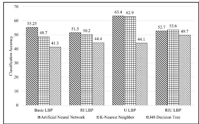
Fig. 2. The Mean or Average Percentage Classification Accuracy of the Standard Classifier Across all LBP Variants (RI LBP = Rotation Invariant LBP, U LBP = Uniform LBP, RIU LBP = Rotation Invariant Uniform LBP).
