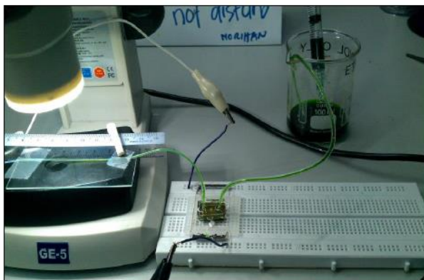
Figure 9: Actual functionality test of thermo pneumatic micropump
