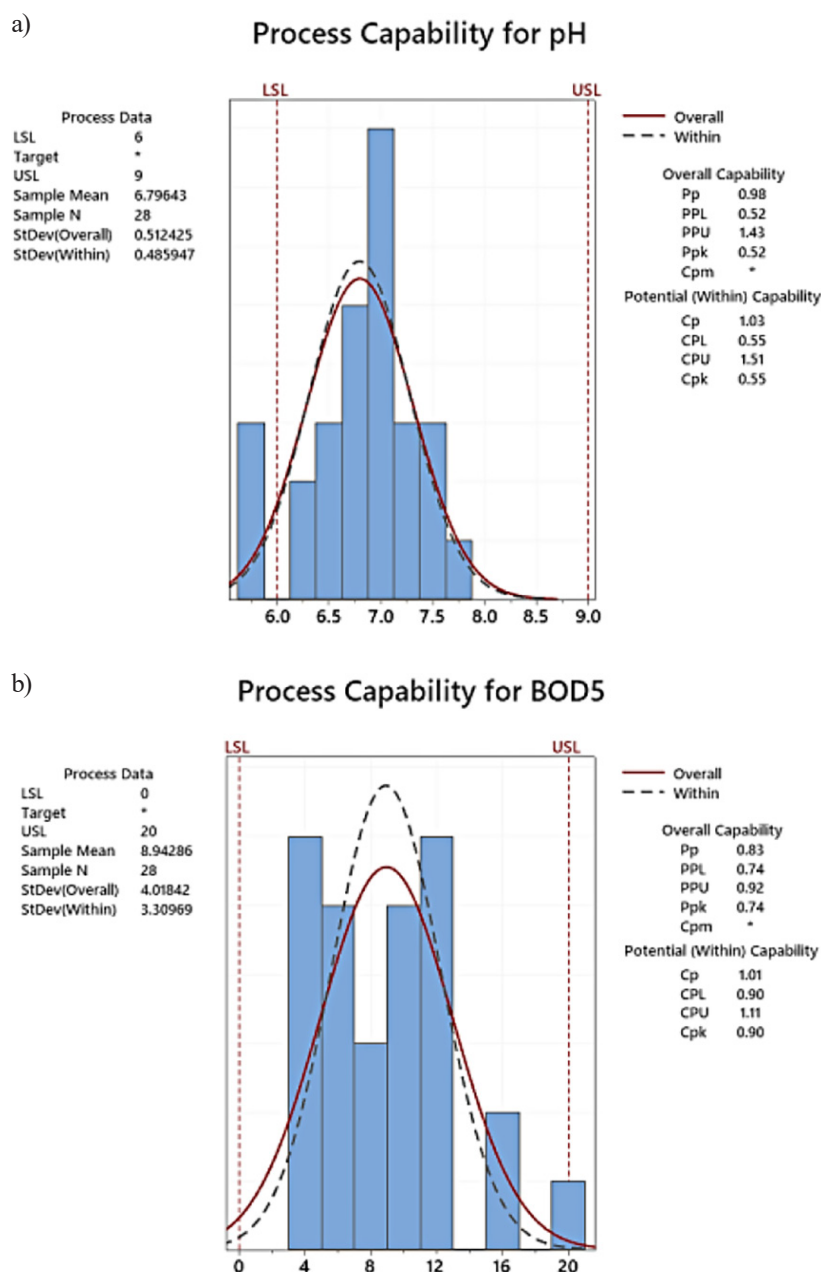
Fig. 3. Process capability for the assessed parameters
