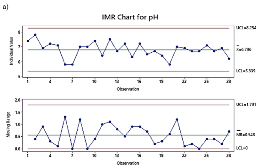
Fig. 2. I-MR control charts for the assessed parameters
