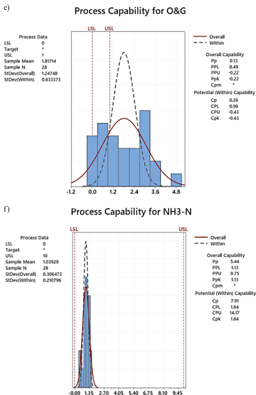
Fig. 3. Cont. Process capability for the assessed parameters
