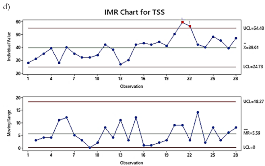
Fig. 2. Cont. I-MR control charts for the assessed parameters
