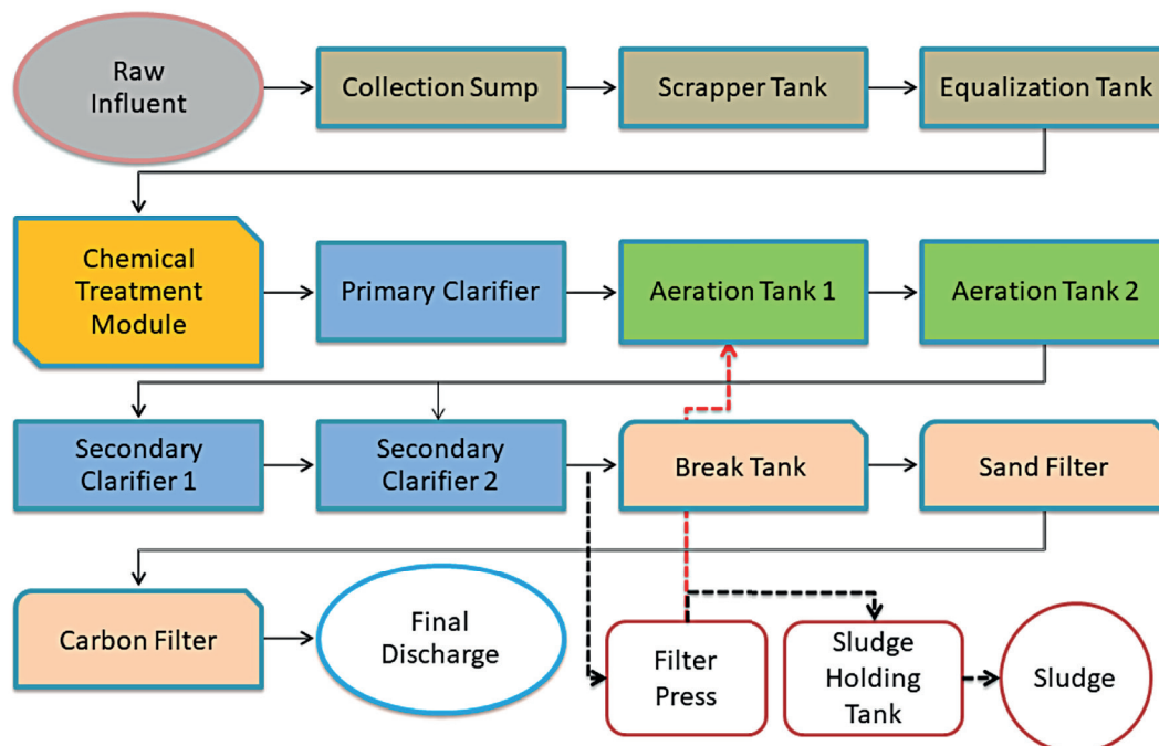
Fig. 1. PWW treatment process
