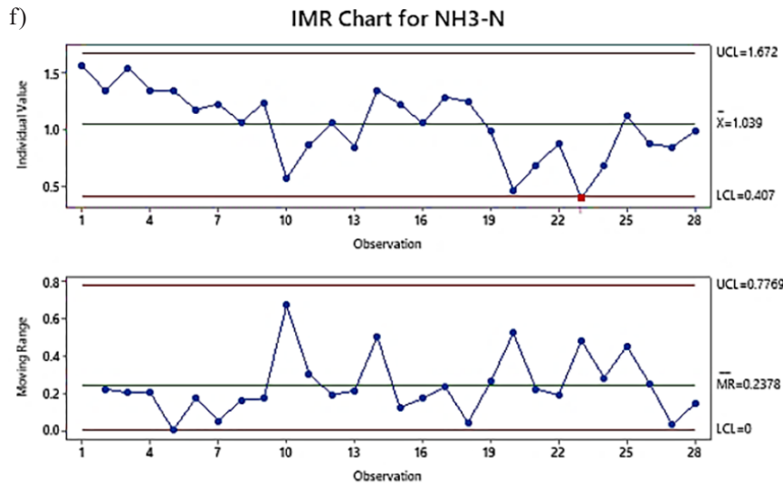
Fig. 2. Cont. I-MR control charts for the assessed parameters
