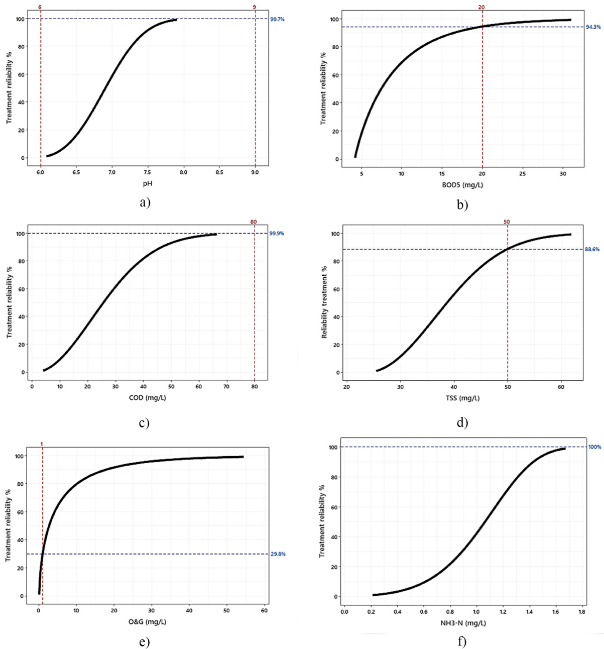
Fig. 4. Weibull cumulative distribution functions and treatment reliability for the assessed parameters
