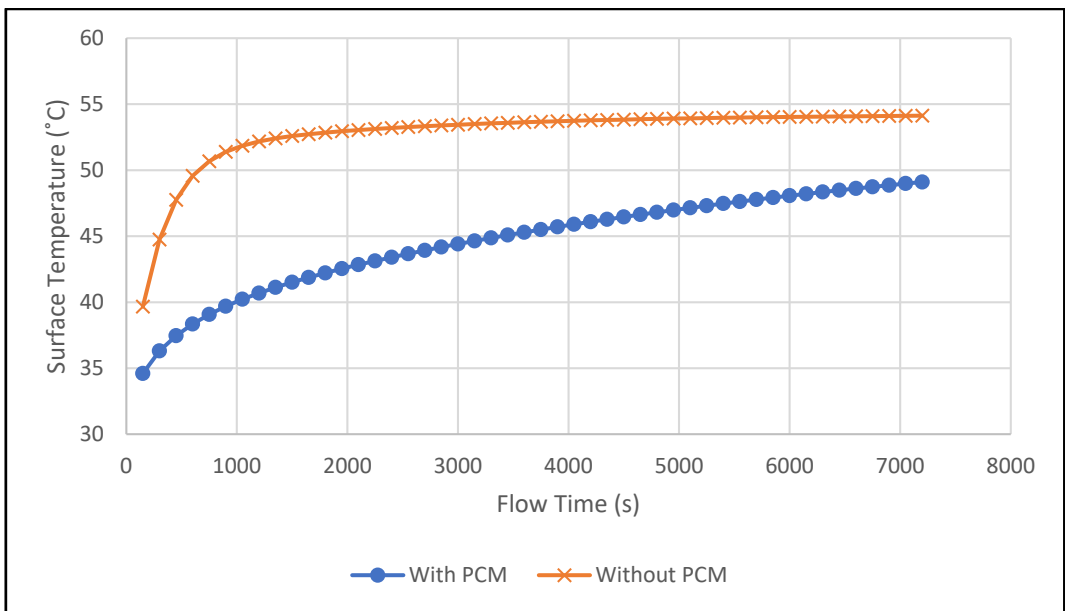
Fig. 9. Comparison of Surface Temperature between PVT and PVT-PCM
