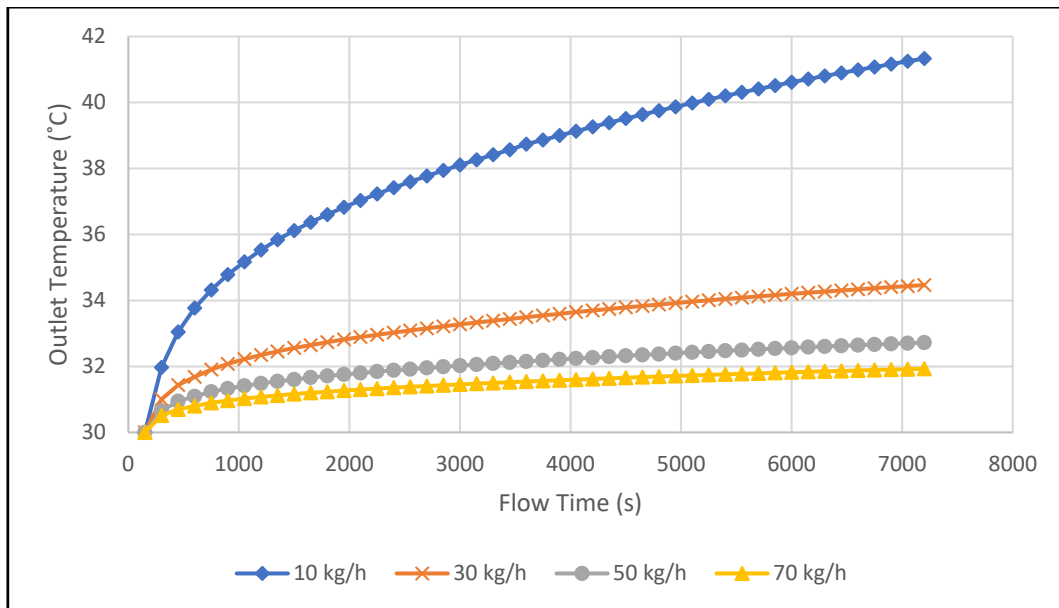
Fig. 4. Outlet Temperature of PVT-PCM on Various Mass Flow Rate at Constant Solar Irradiance 450 \text{ W/m}^2
