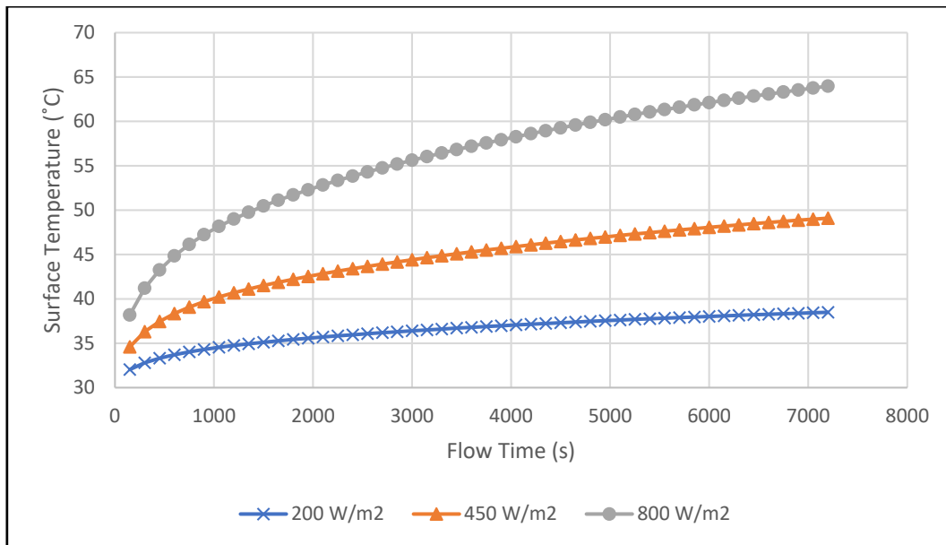
Fig. 6. Surface Temperature on Various Solar Irradiance at Constant Mass Flow Rate 10kg/h
