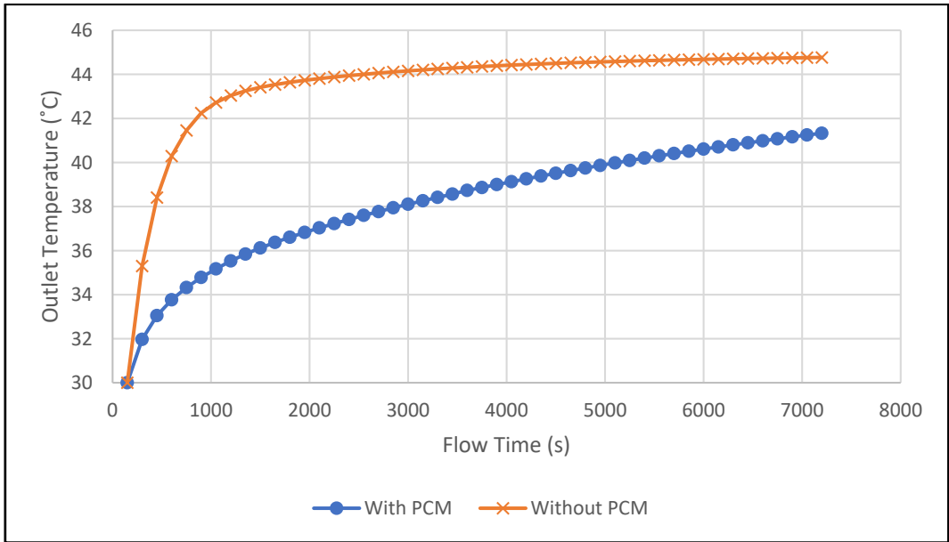
Fig. 8. Comparison of Outlet Temperature between PVT and PVT-PCM
