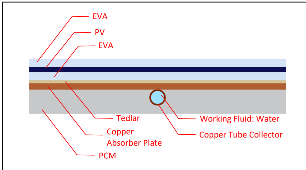
Fig. 2. Cross section of PVT-PCM model
