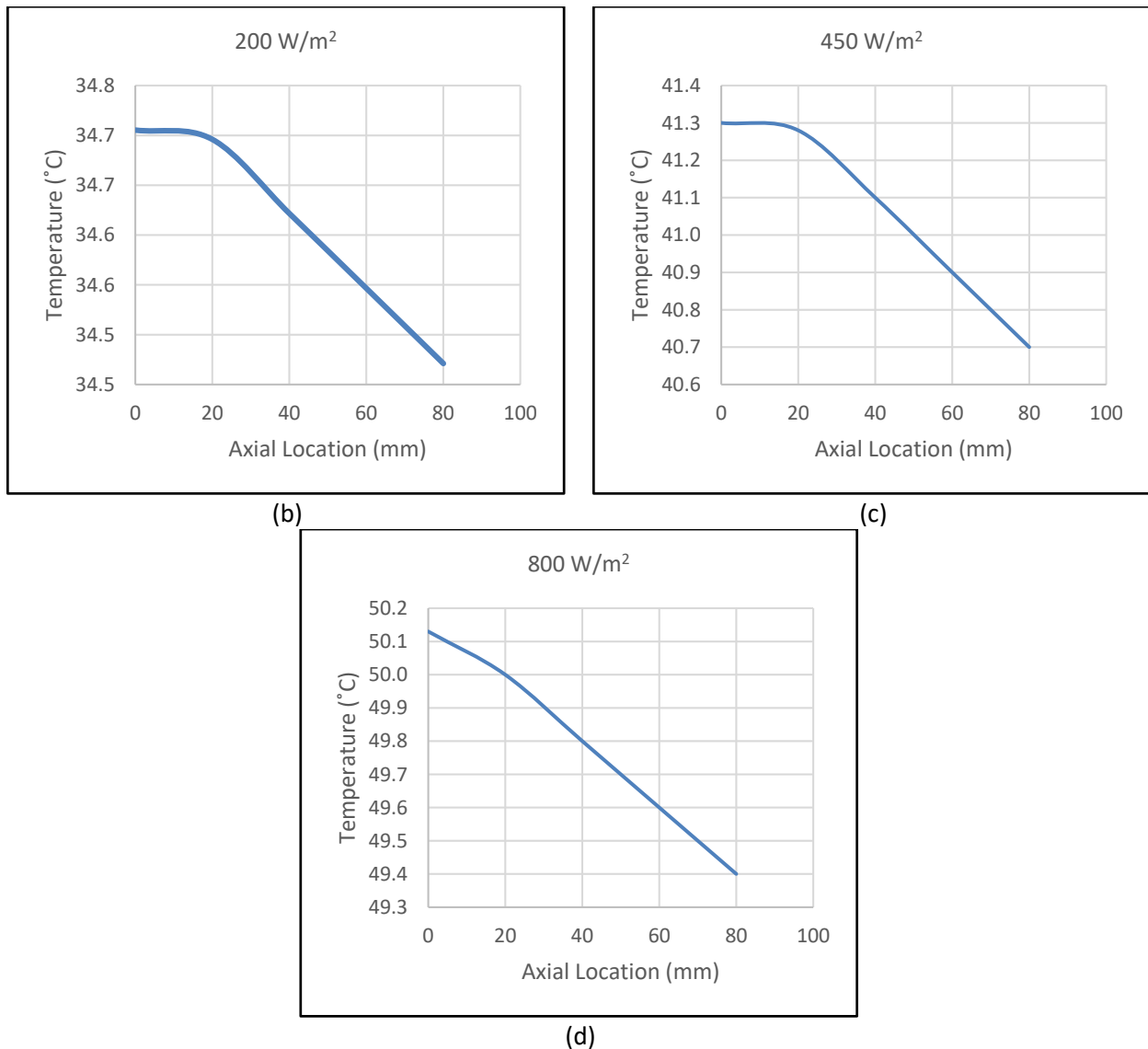
Fig. 7. (a) Axial Temperature Distribution (b) Axial Temperature Profile at 200 W/m 2 (c) Axial Temperature Profile at 450 W/m 2 (d) Axial Temperature Profile at 800 W/m 2
