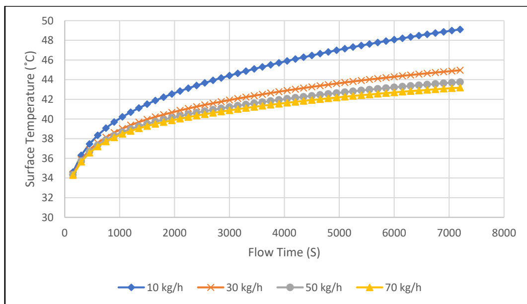
Fig. 3. Surface Temperature of PVT-PCM on Various Mass Flow Rate at Constant Solar Irradiance 450 W/m 2
