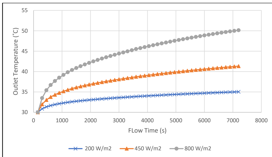
Fig. 5. Outlet Temperature on Various Solar Irradiance at Constant Mass Flow Rate 10kg/h
