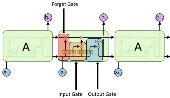
Fig. 3. LSTM Gates [29].
