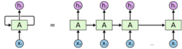
Fig. 4. An Unrolled RNN [29].
