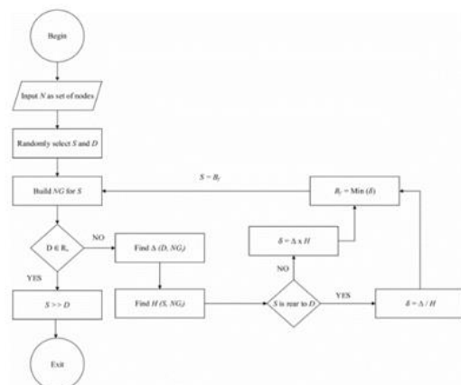
Figure 11: DBAFS protocol [45].
