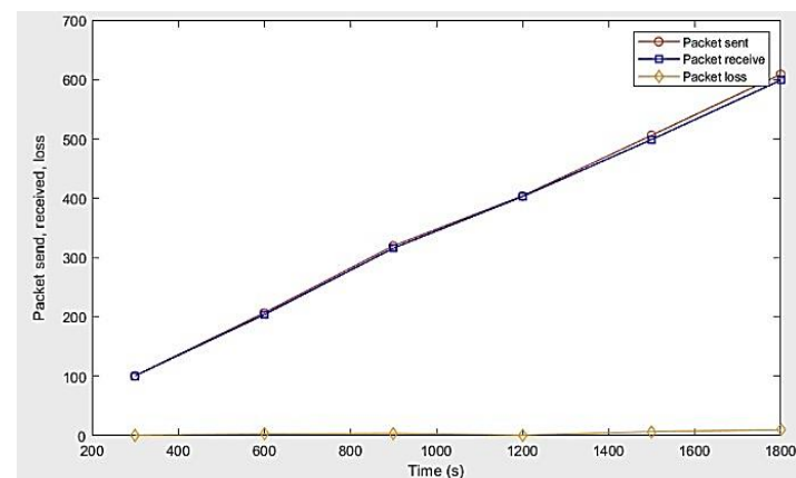
Figure 5. Packet loss from the simulation result
