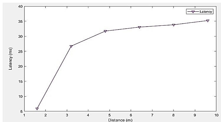
Figure 7. Latency from the simulation result
