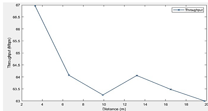
Figure 11. Throughput from the measurement result
