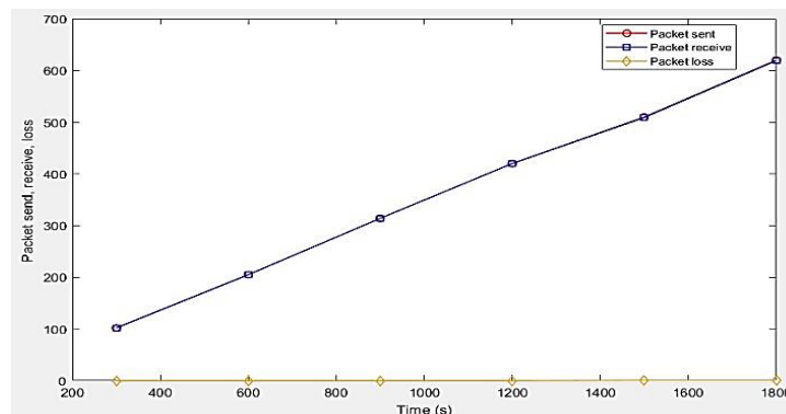
Figure 14. Packet loss from the measurement result
