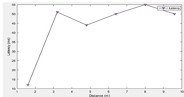
Figure 8. Latency from the measurement result
