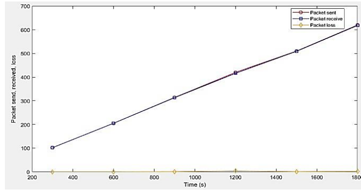
Figure 15. Packet loss from the simulation result
