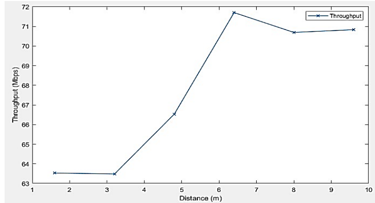
Figure 6. Throughput from the measurement result
