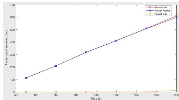
Figure 17. Packet loss from the measurement result
