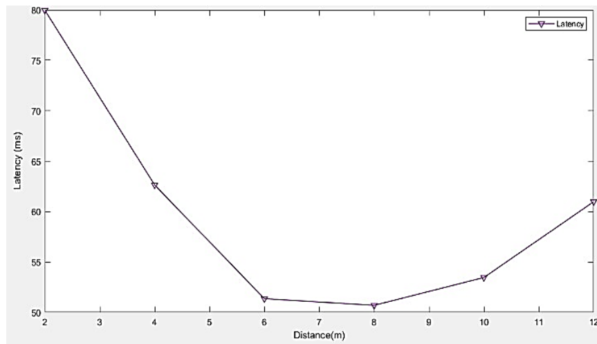
Figure 19. Latency from the measurement result
